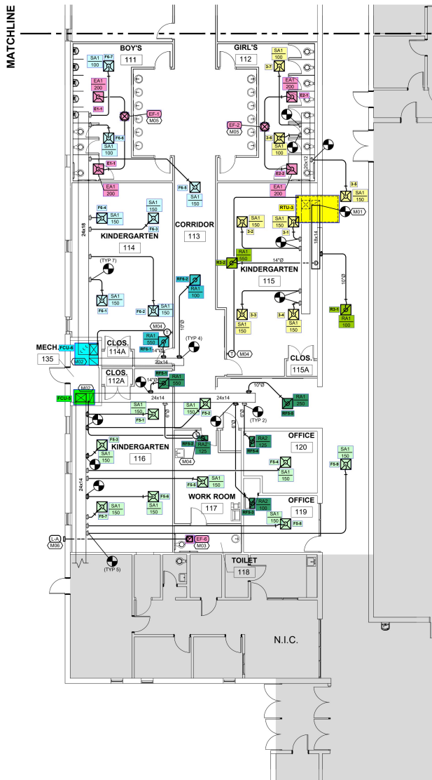
LEVEL 1 FLOOR PLAN - AREA B - MECHANICAL NEW WORK SCALE: 1/8" = 1'-0"
