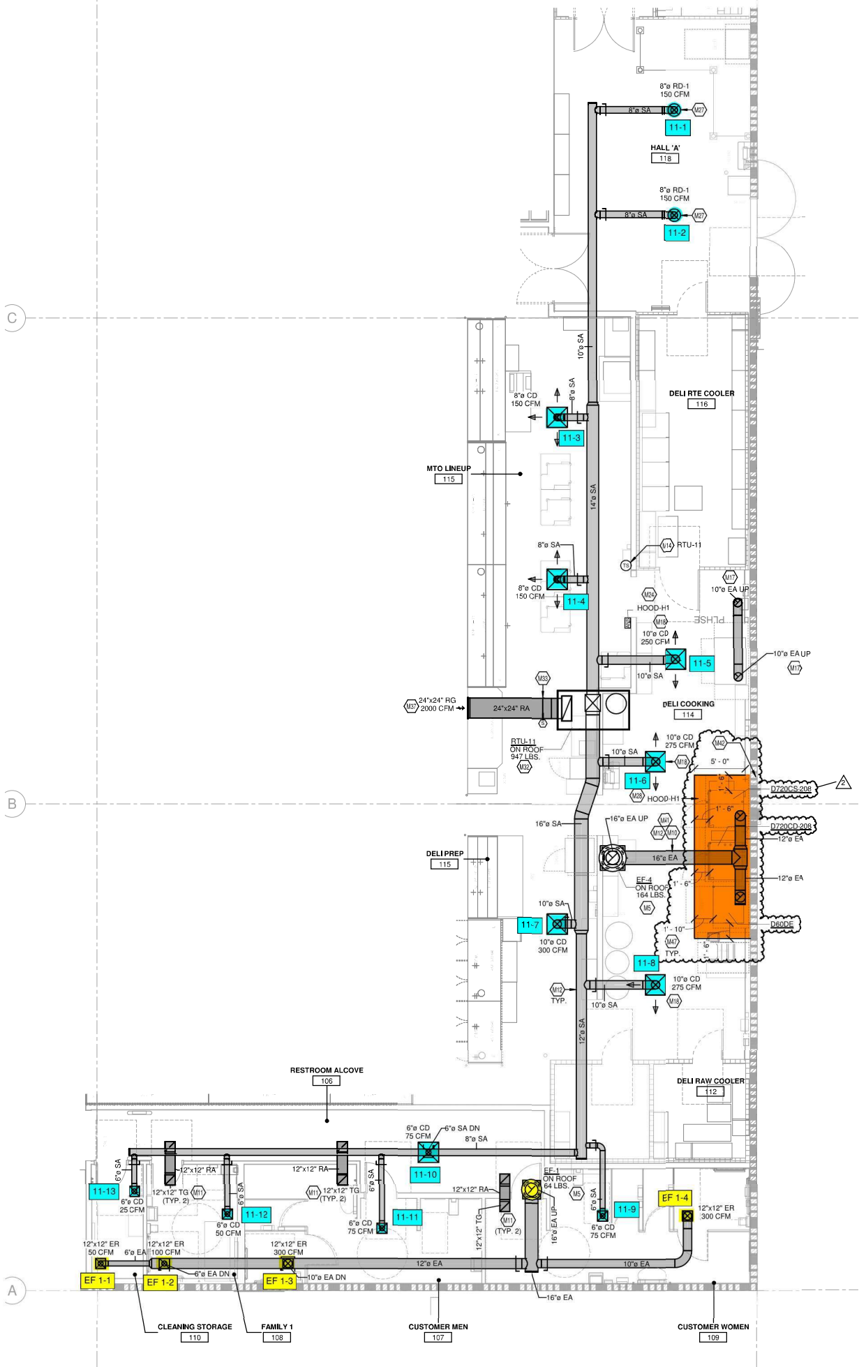
HVAC ENLARGED PLAN - DELI 3/16" = 1'-0"
