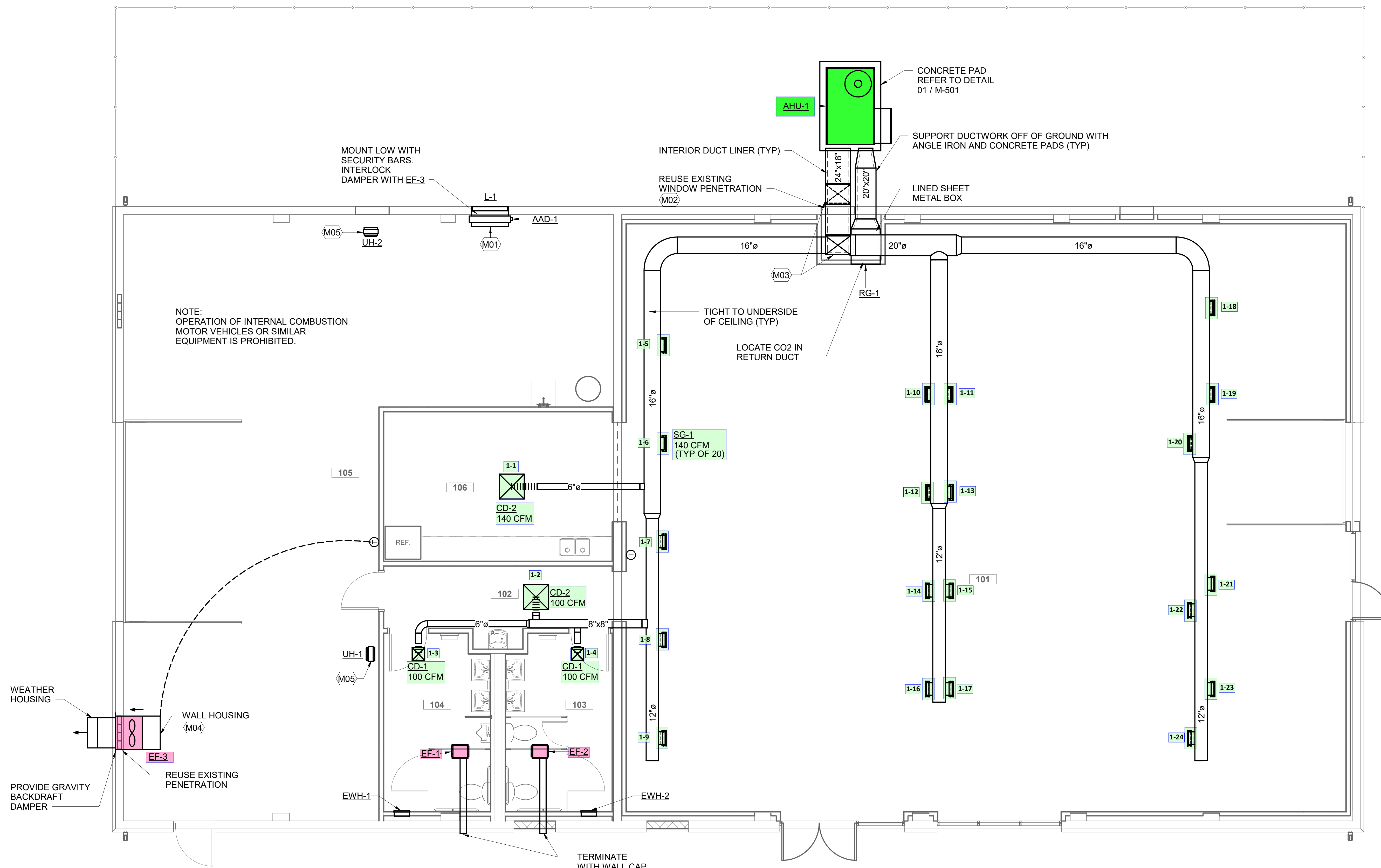
01 MECHANICAL FLOOR PLAN M-101 1/4" = 1'-0"
