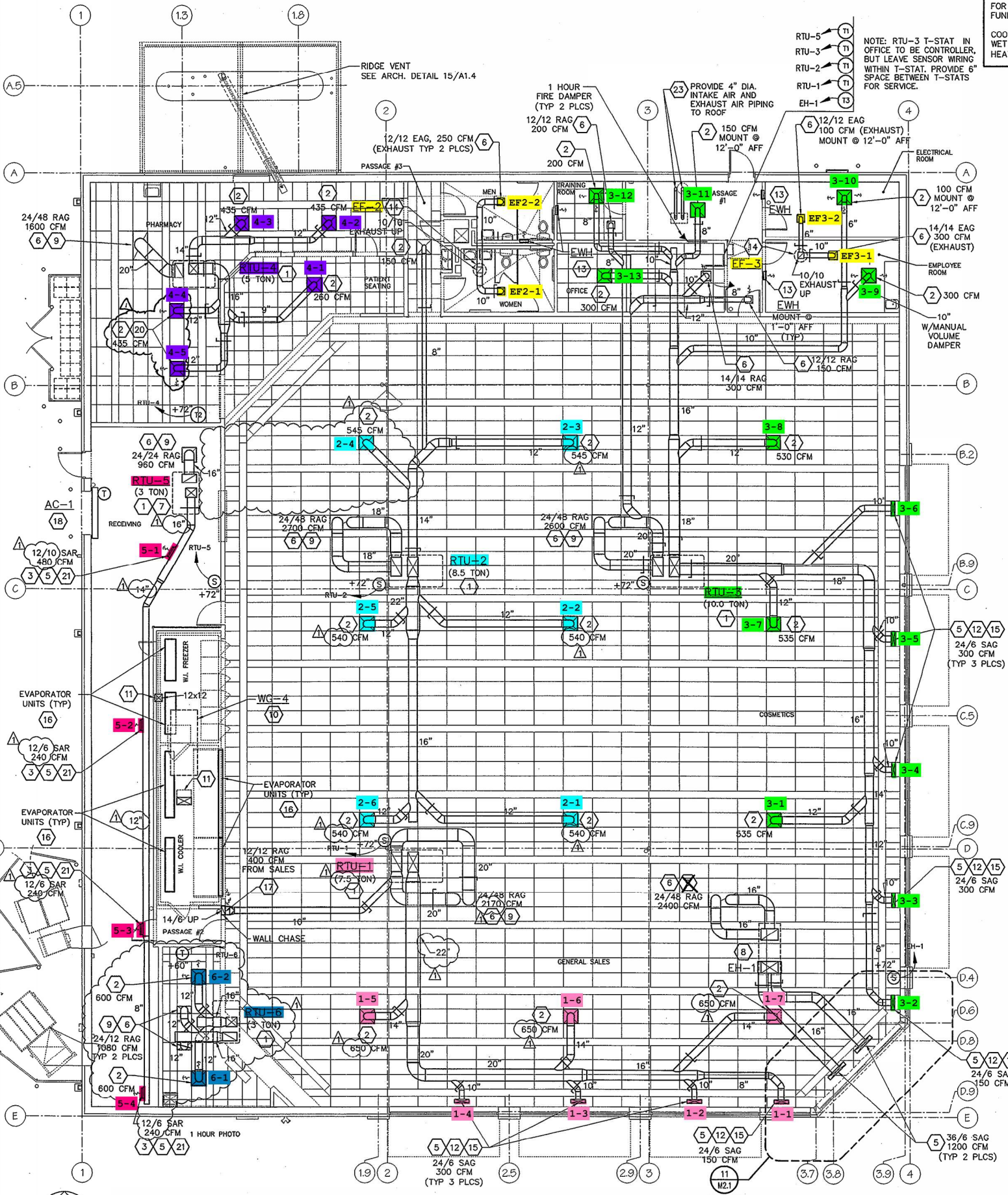
FLOOR PLAN - MECHANICAL SCALE: 1/8"=1'-0"
