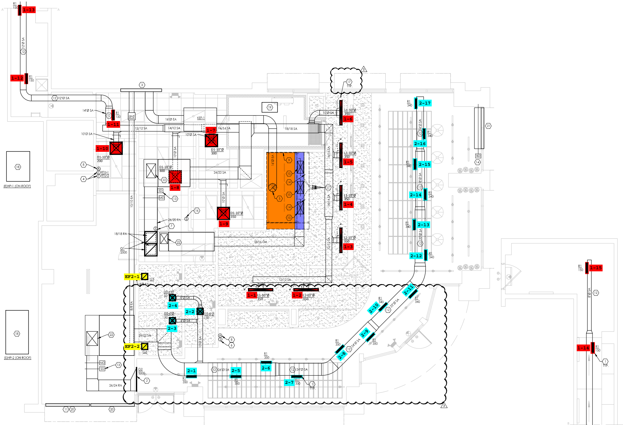
1 MECHANICAL PLAN 1/4" = 1'-0"
