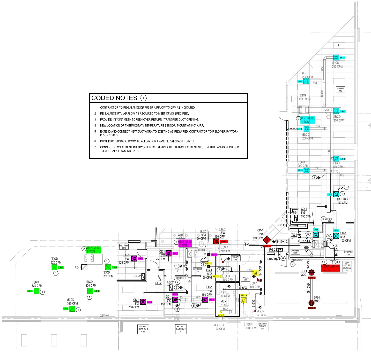
MECHANICAL NEW PLAN SCALE: 1/8" = 1'-0"
