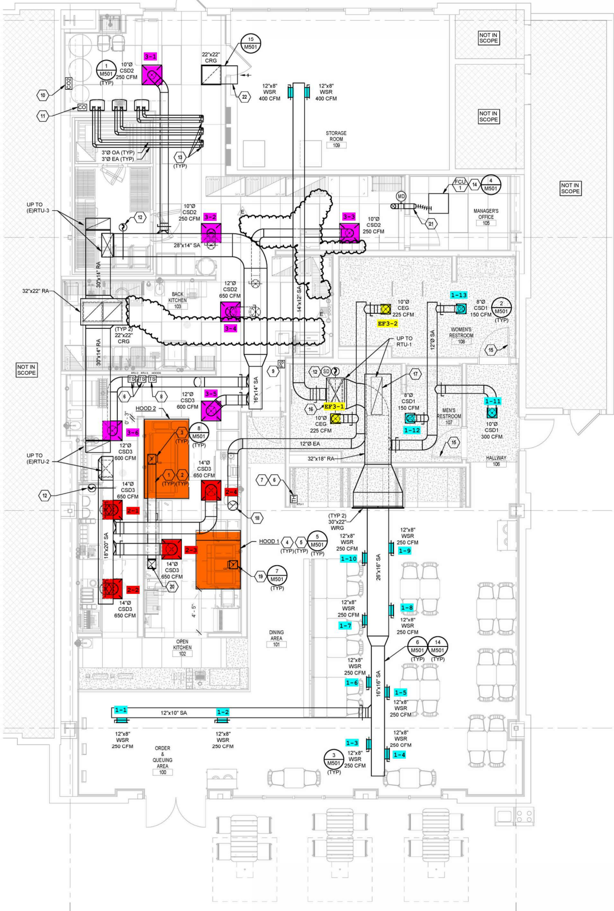
1 MECHANICAL FLOOR PLAN 1/4" = 1'-0"
