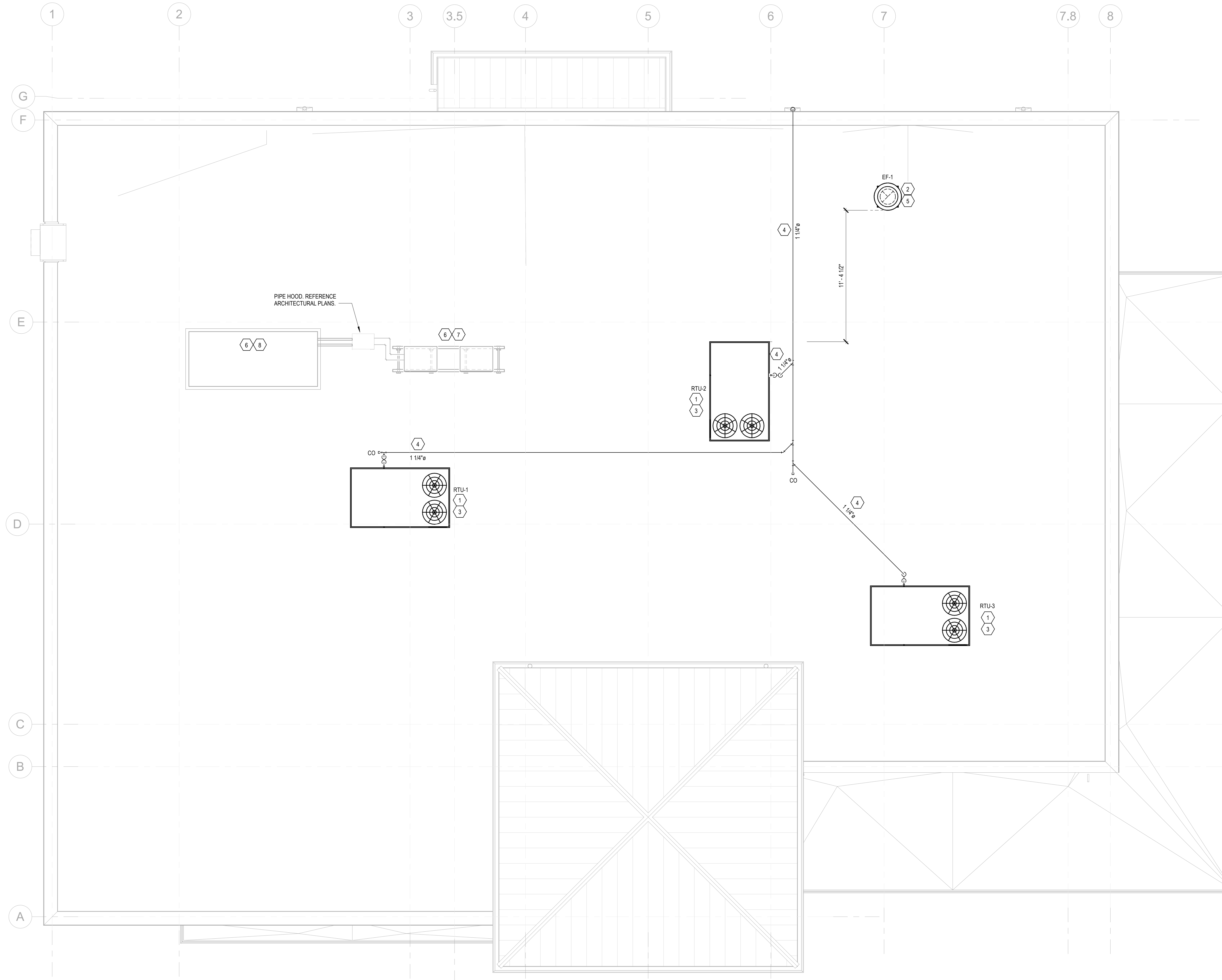
1 HVAC ROOF PLAN M2.0 1/4" = 1'-0"
