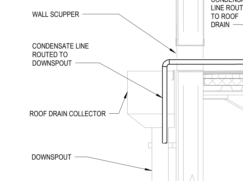
8 CONDENSATION TERMINATION DETAIL M3.0 NOT TO SCALE
