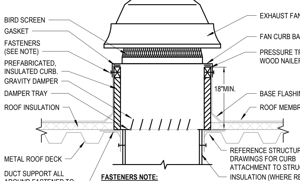
7 ROOF FAN MOUNTING DETAIL M3.0 NOT TO SCALE
