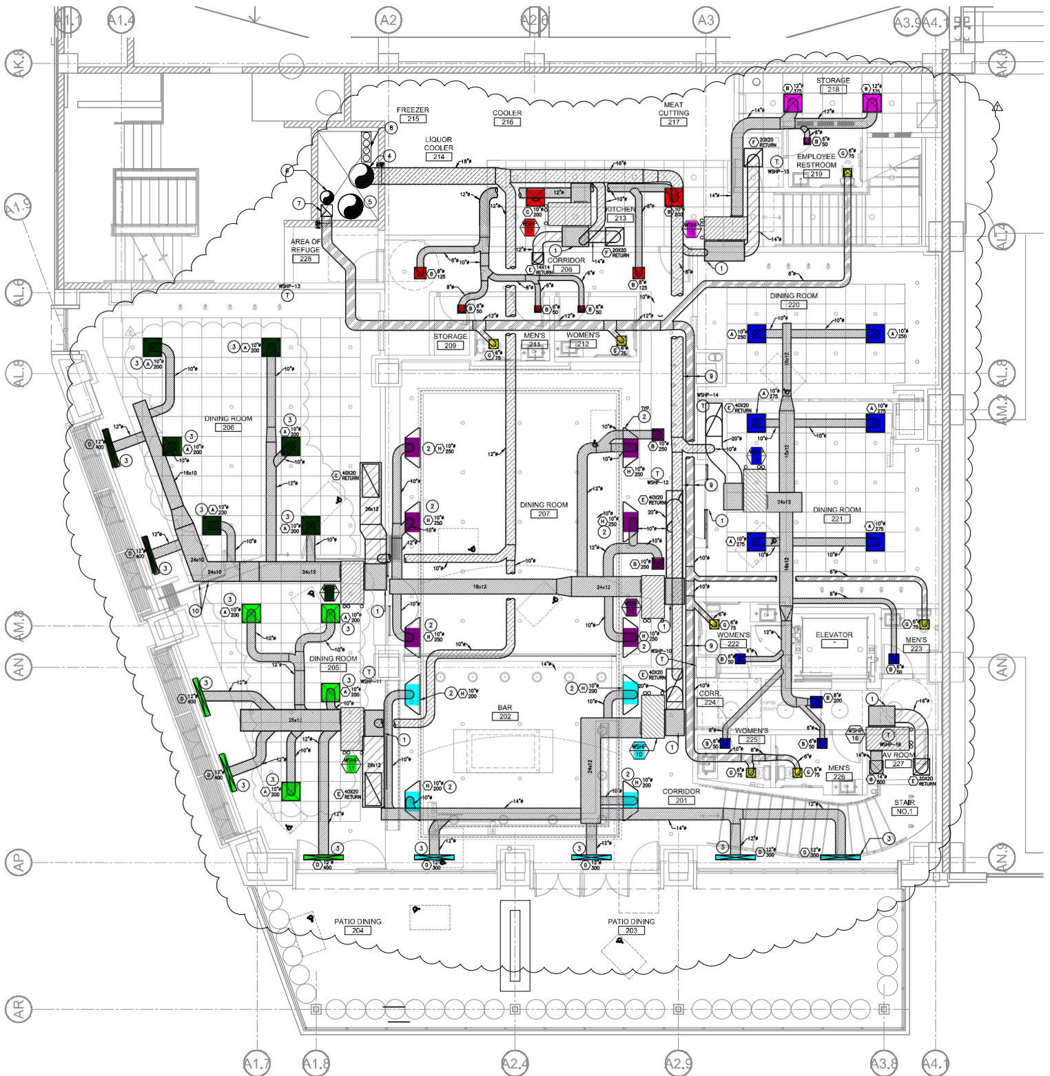
2ND FLOOR MECHANICAL PLAN 1/4"=1'-0"
