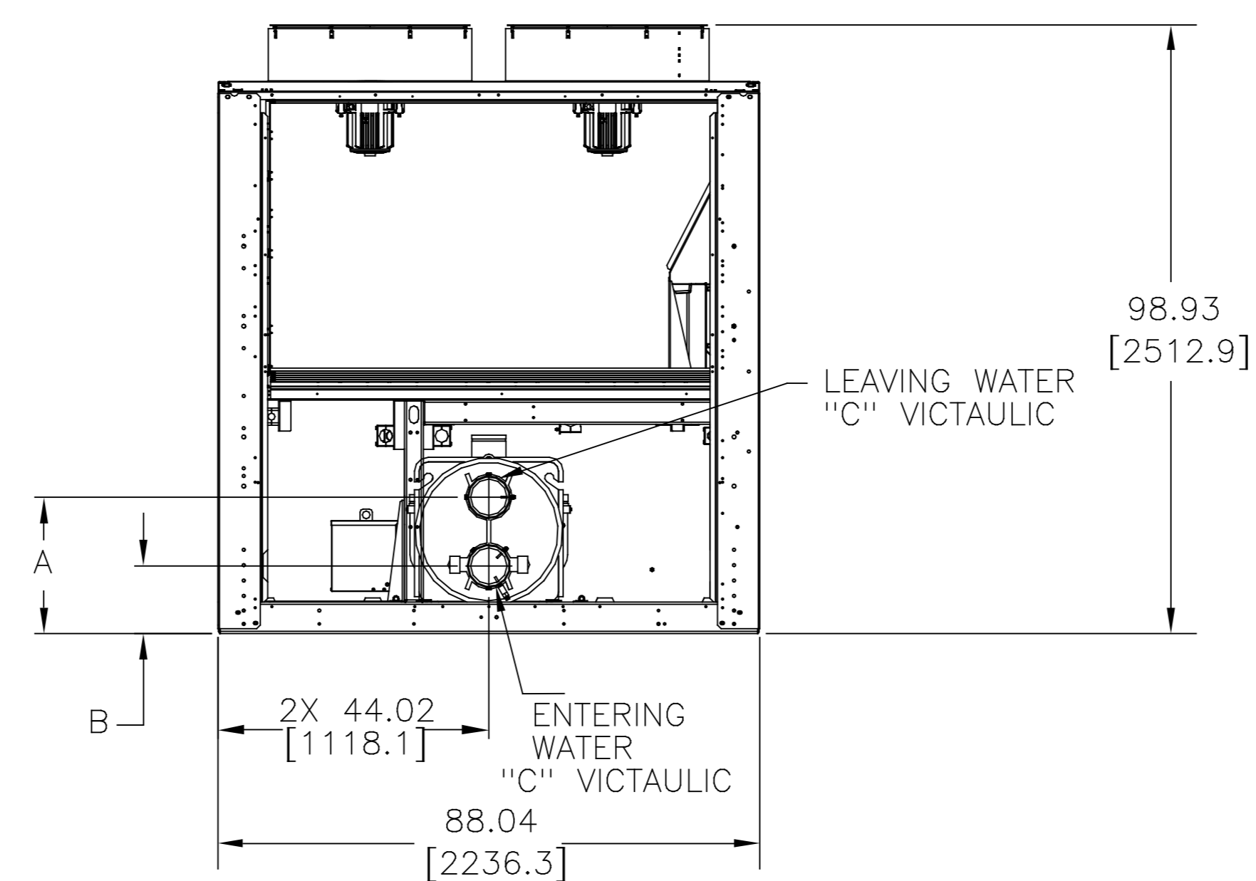
FLOODED EVAPORATOR, 2 PASS
