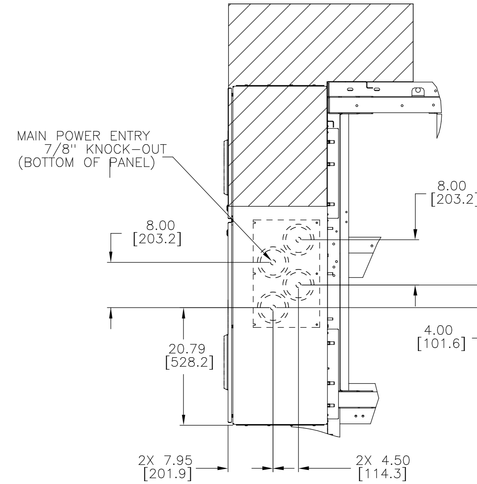
DETAIL C (TOP VIEW- KNOCK OUTS ON BOTTOM OF CONTROL BOX)
