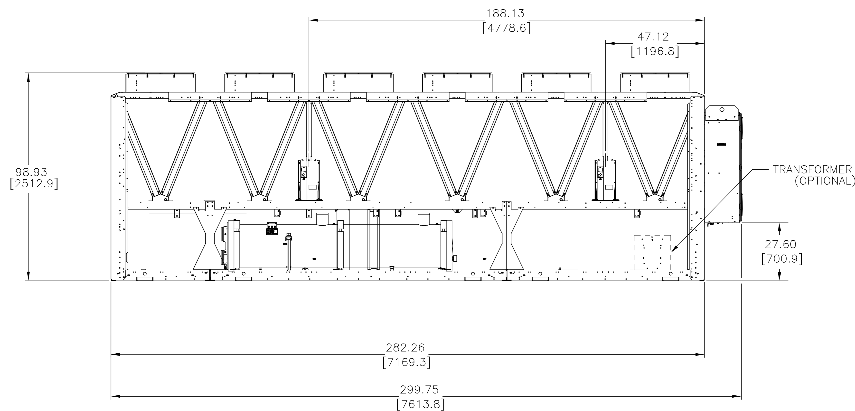
30XV REAR VIEW
