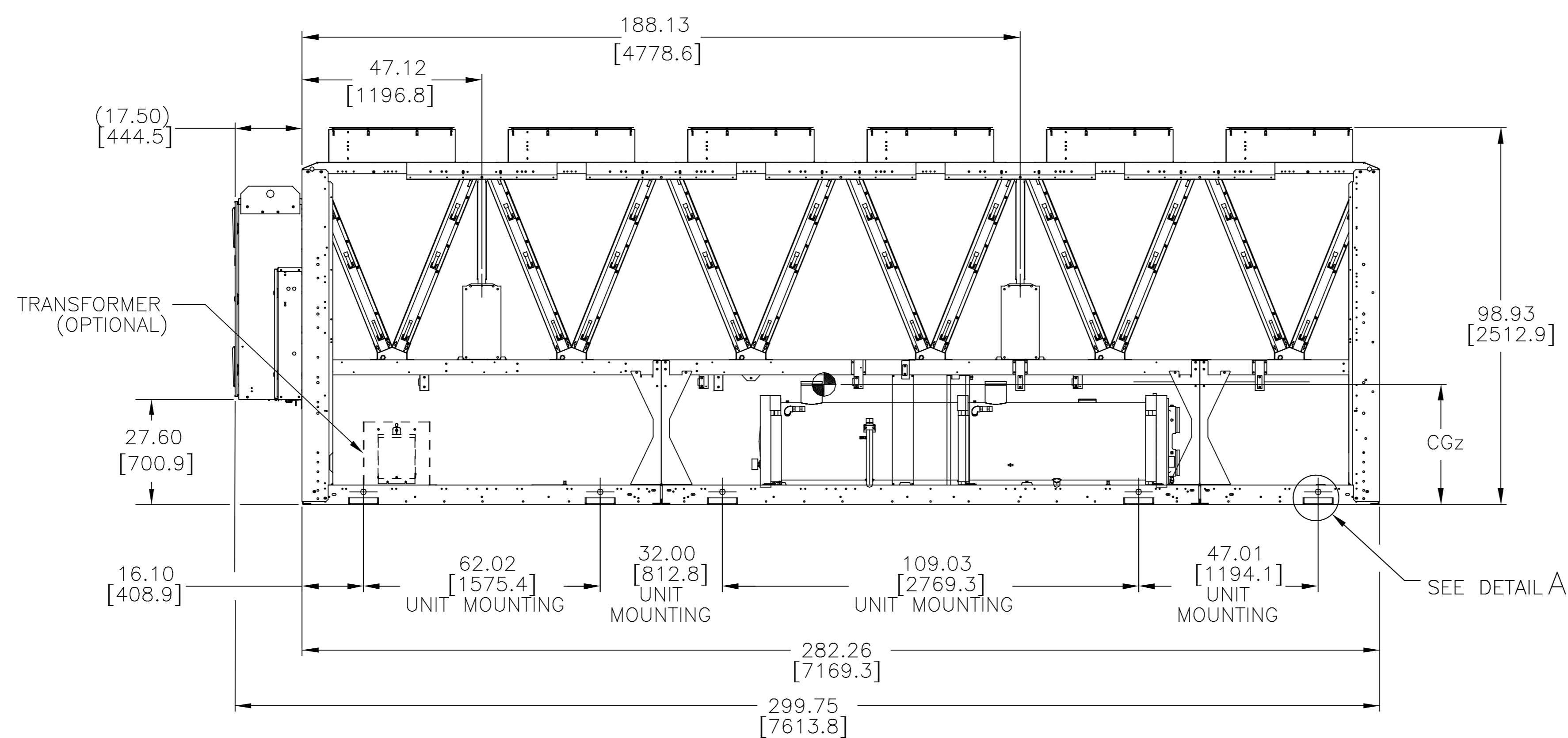
30XV FRONT VIEW (CONDENSER HEADER END)
