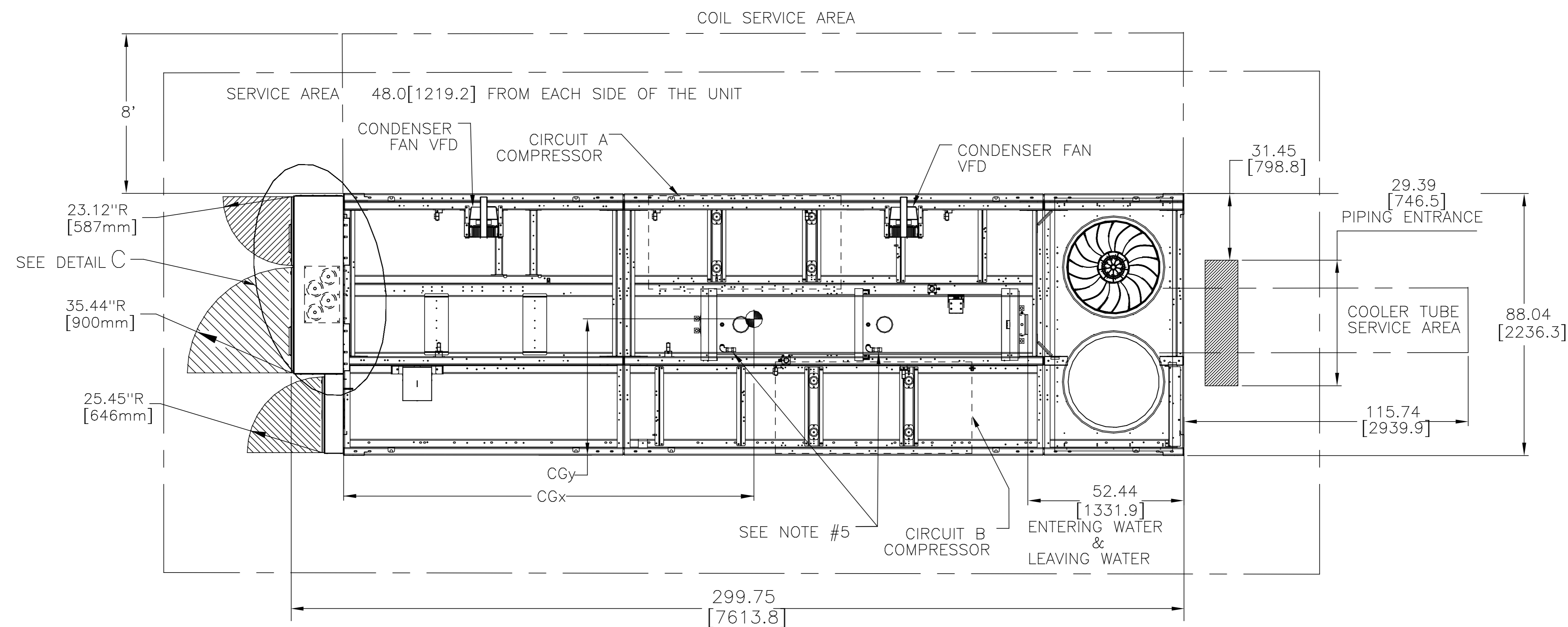
30XV PLAN VIEW
