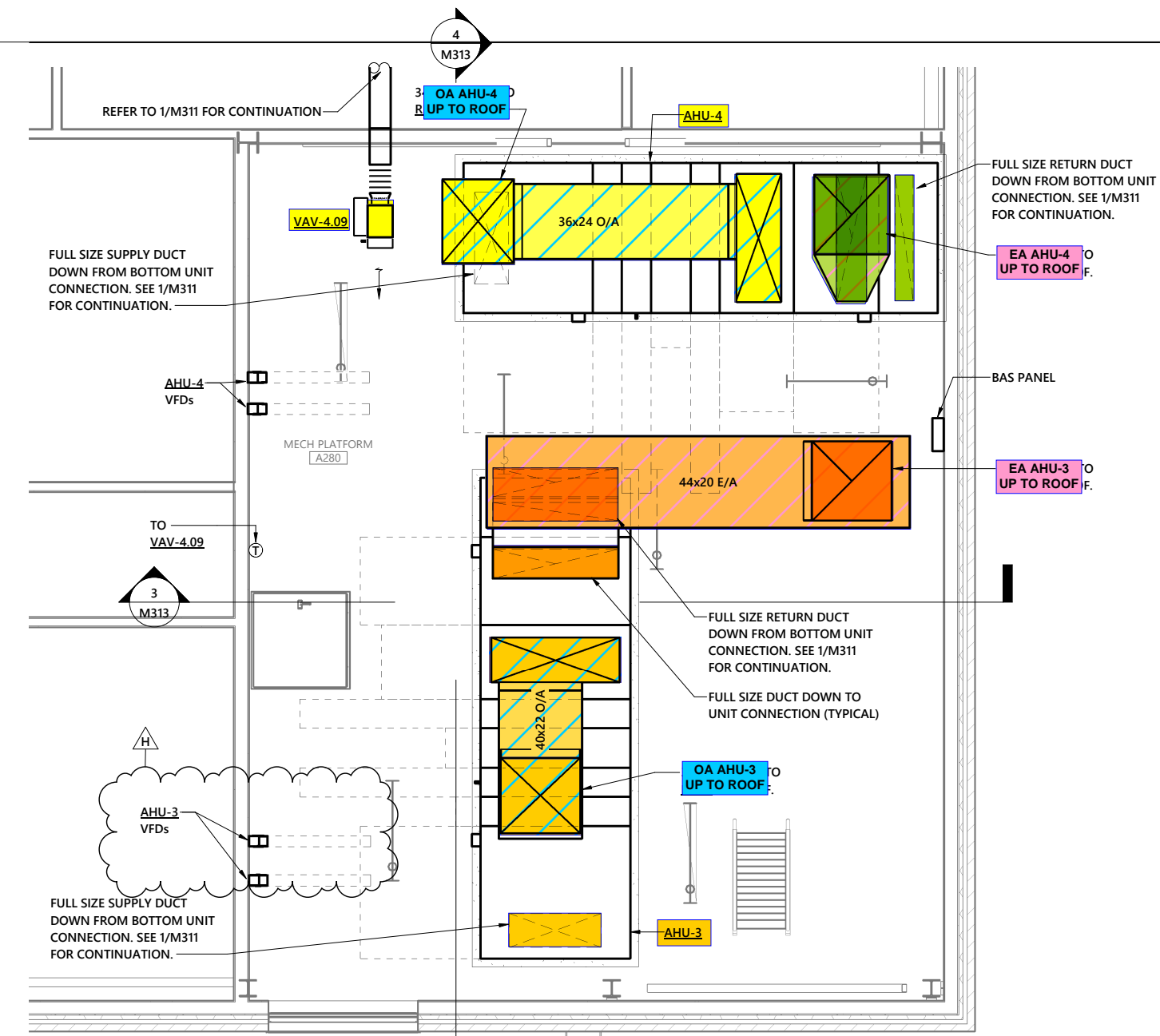
2 ENLARGED MECHANICAL PLAN - MECH PLATFORM A280 1/4" = 1'-0"
