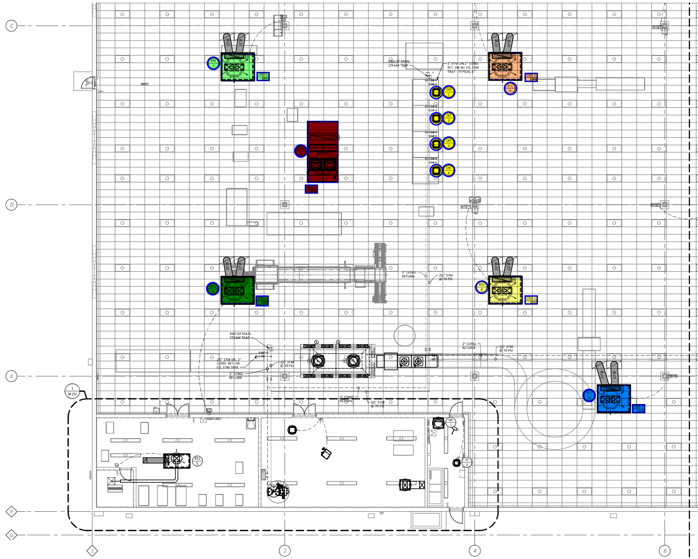
ENLARGED BAKERY MECHANICAL PLAN SCALE: 1/8" = 1'-0"
