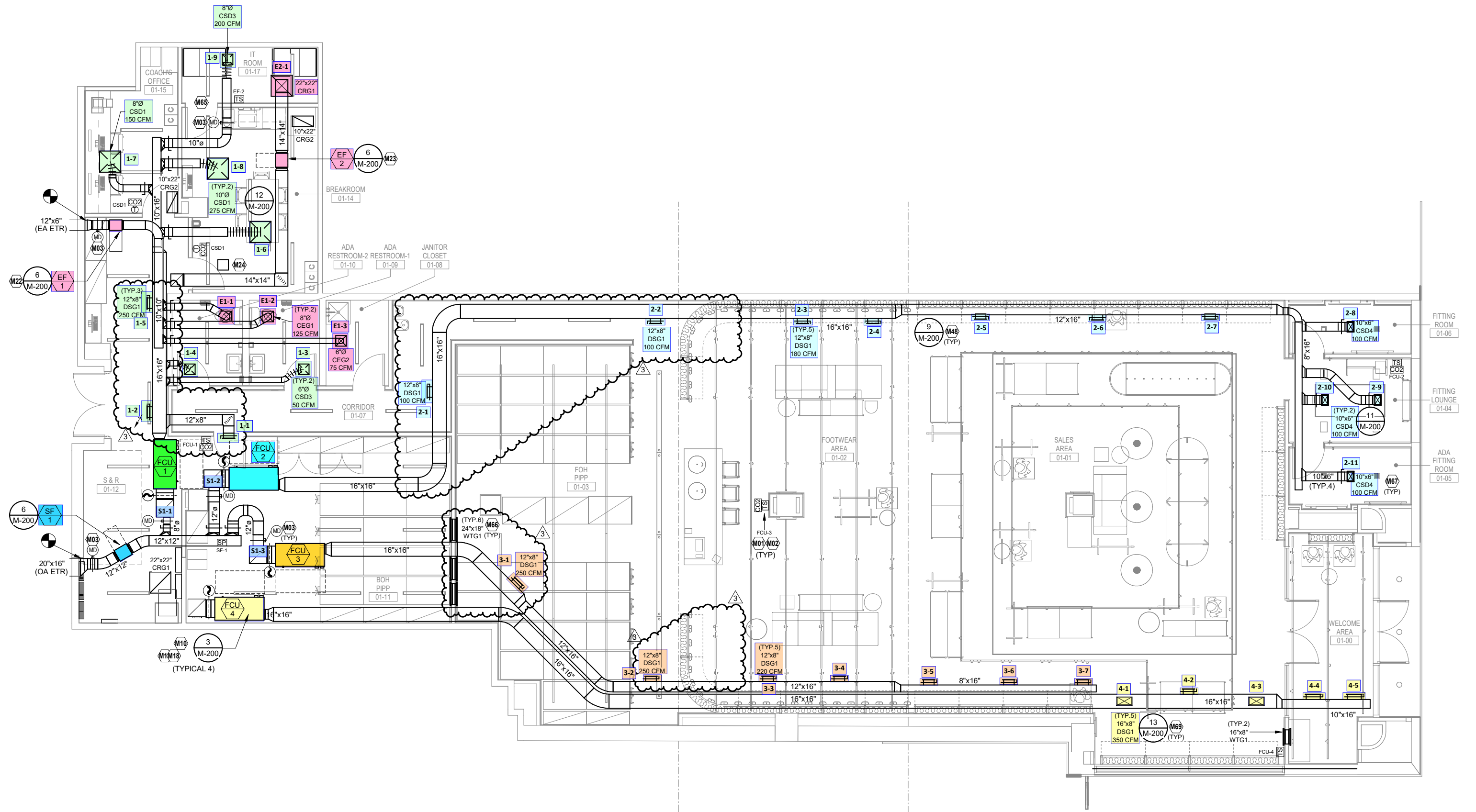
① HVAC PLAN 3/16" = 1'-0"
