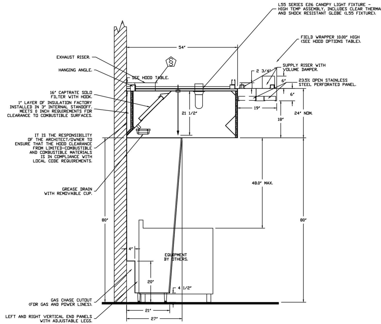
SECTION VIEW - MODEL 5424ND-2-ACPSP-P HOOD - 41
