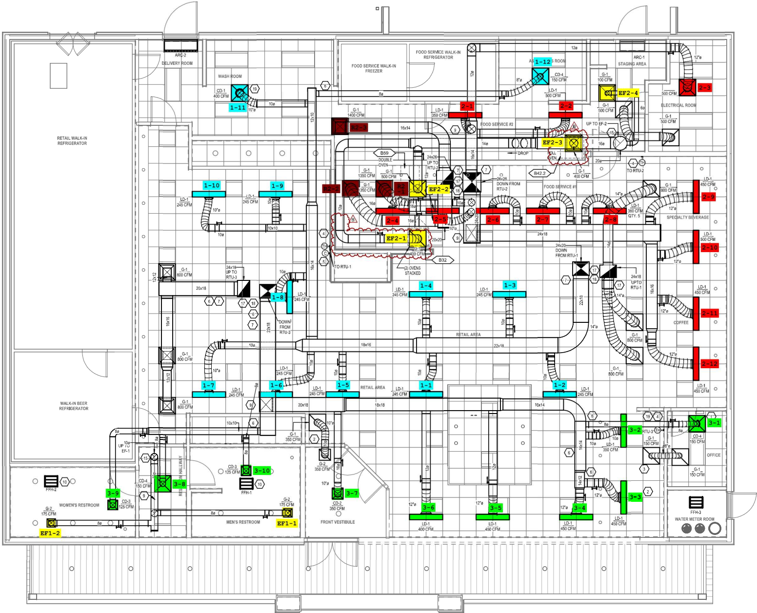
1 HVAC FLOOR PLAN M1.0 1/4" = 1'-0"
