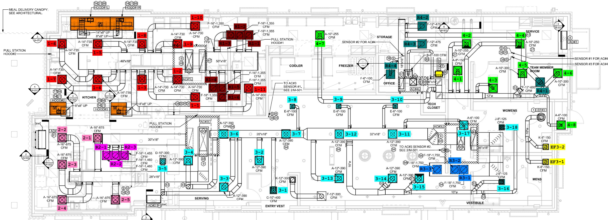
1 EQUIPMENT AND DUCTWORK PLAN 1/4" = 1'-0"
