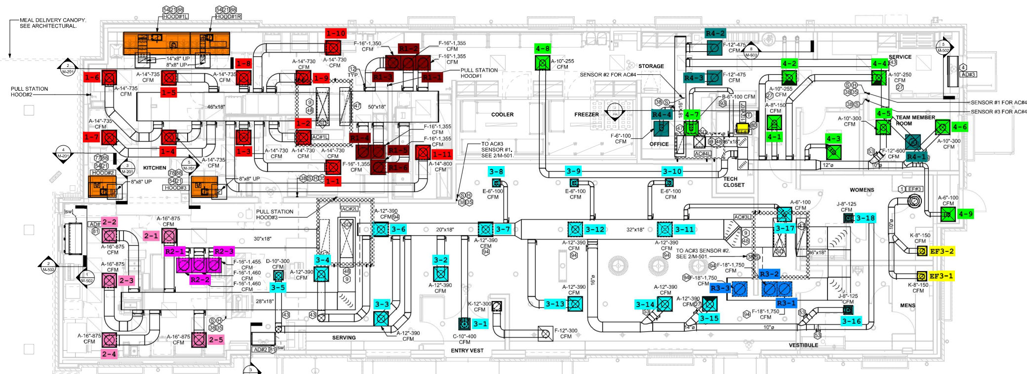
1 EQUIPMENT AND DUCTWORK PLAN 1/4" = 1'-0"
