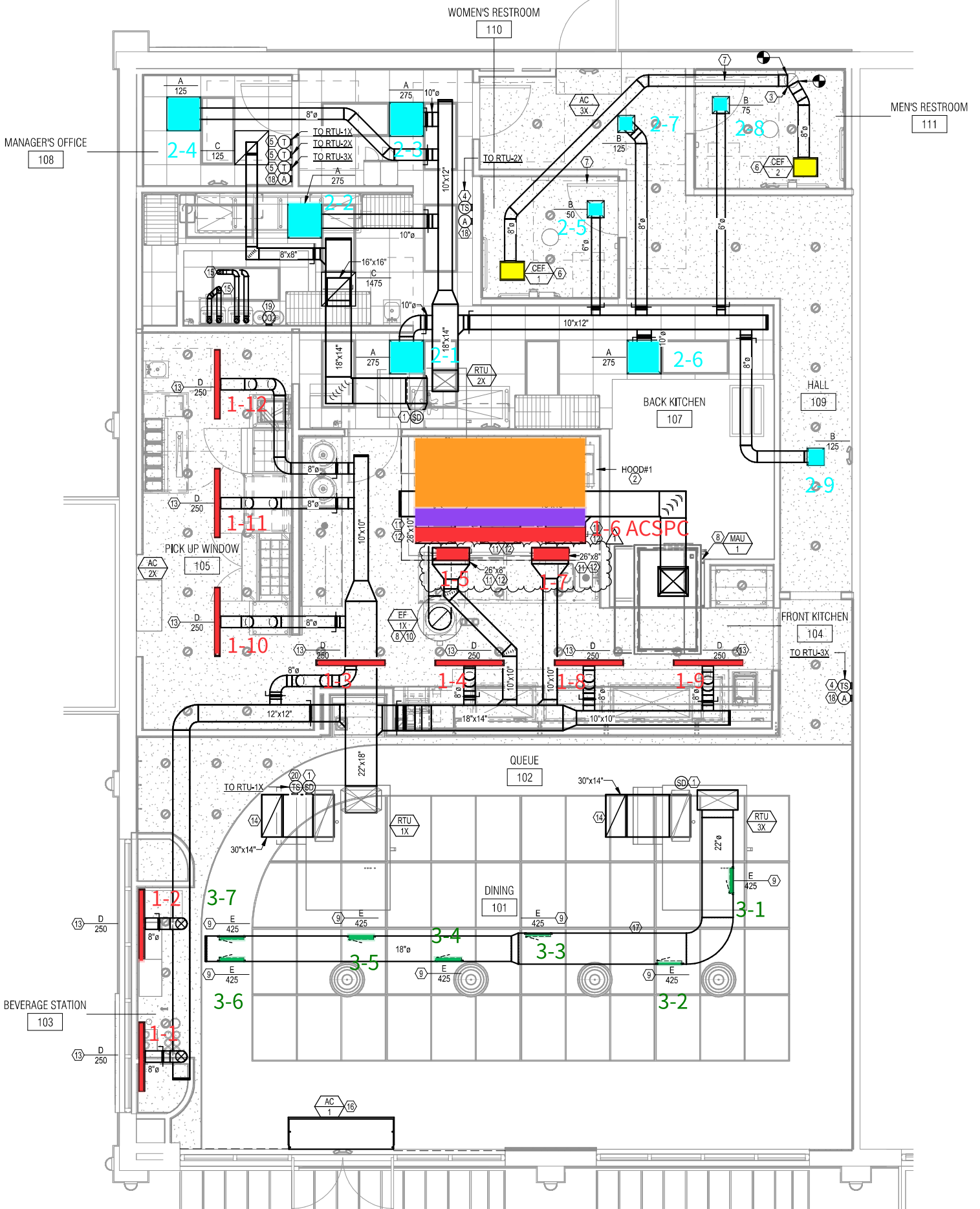
MECHANICAL PLAN SCALE: 1/4" = 1'-0"
