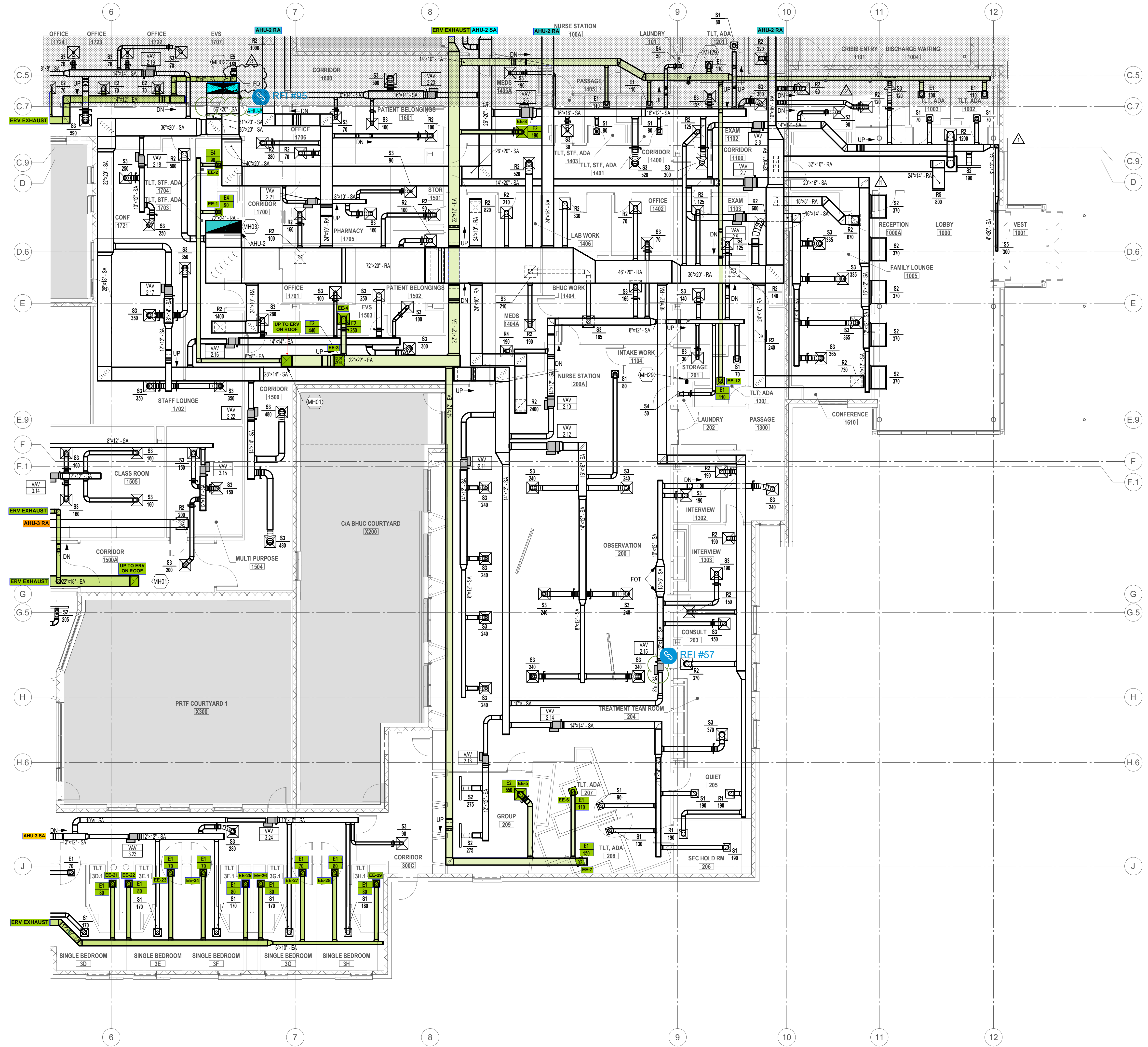
1 MECHANICAL FLOOR PLAN - AREA A - HVAC 1/8" = 1'-0"
