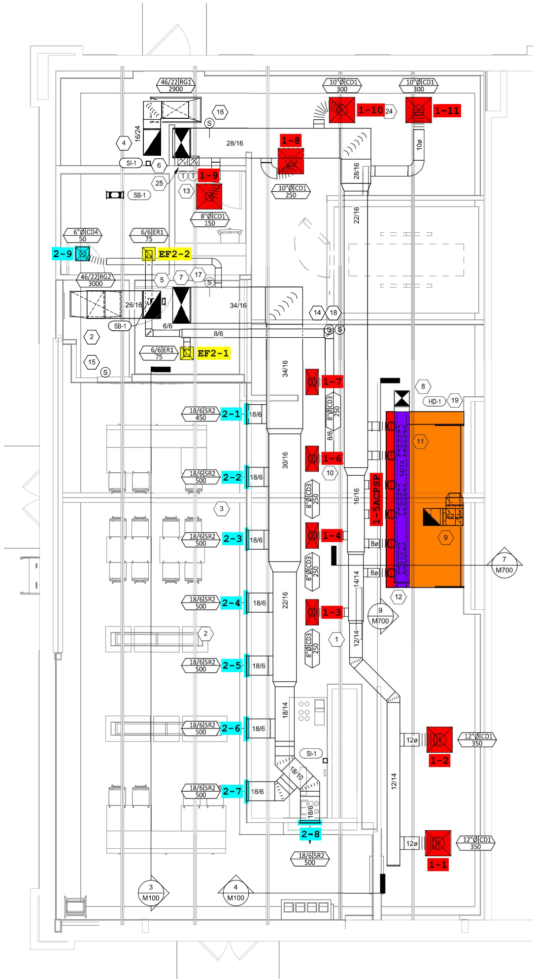
HVAC FLOOR PLAN
