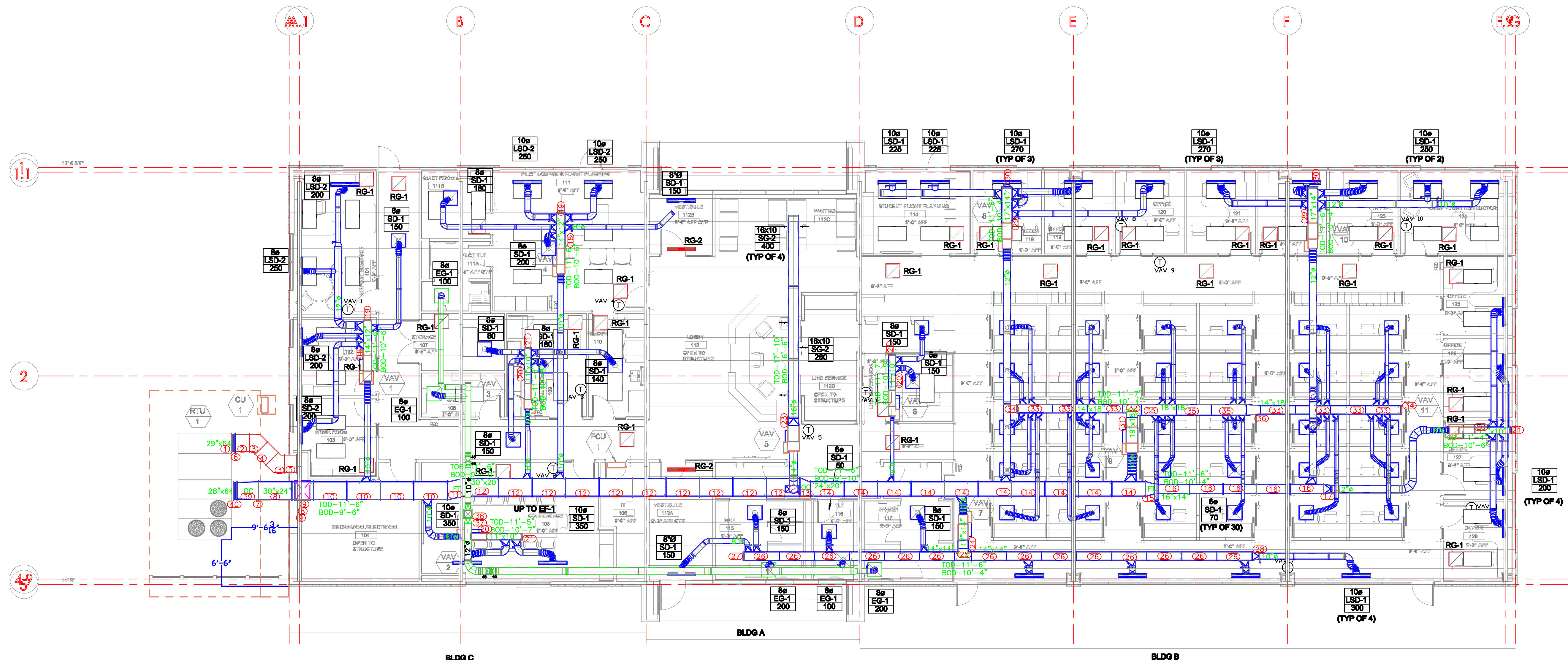
LEVEL 1 - HVAC PLAN
