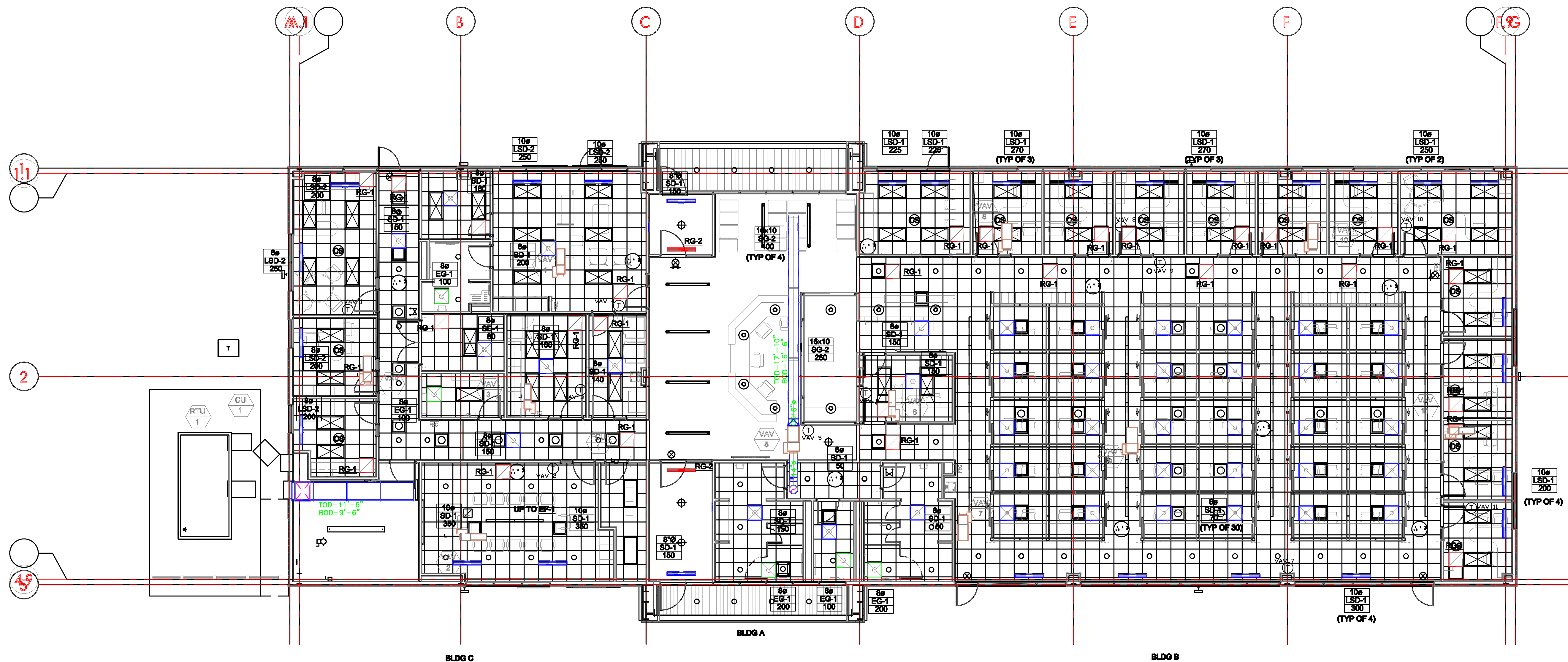
LEVEL 1 - REFLECTIVE CEILING PLAN
