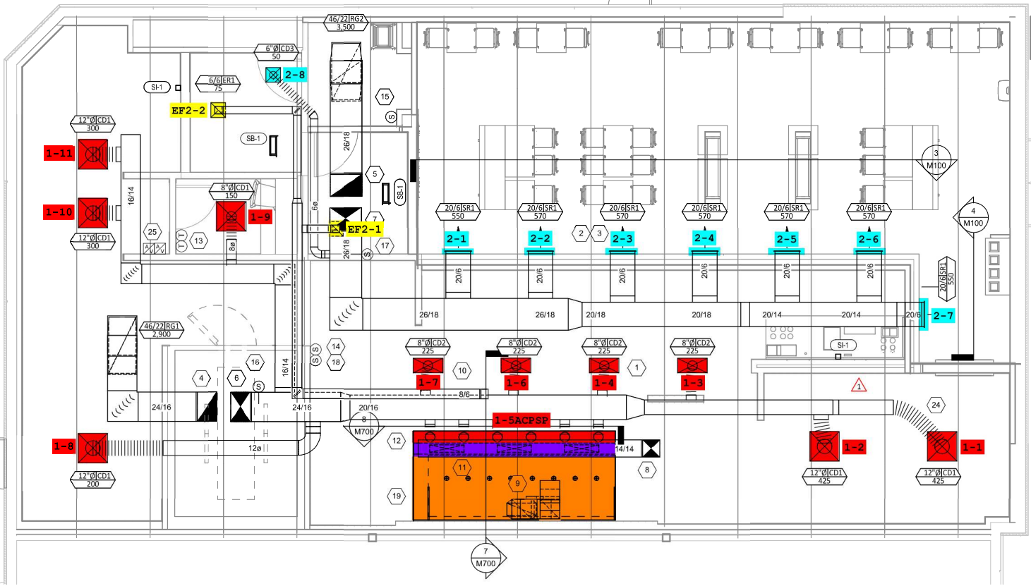
M100 1/4" = 1'-0" HVAC FLOOR PLAN
