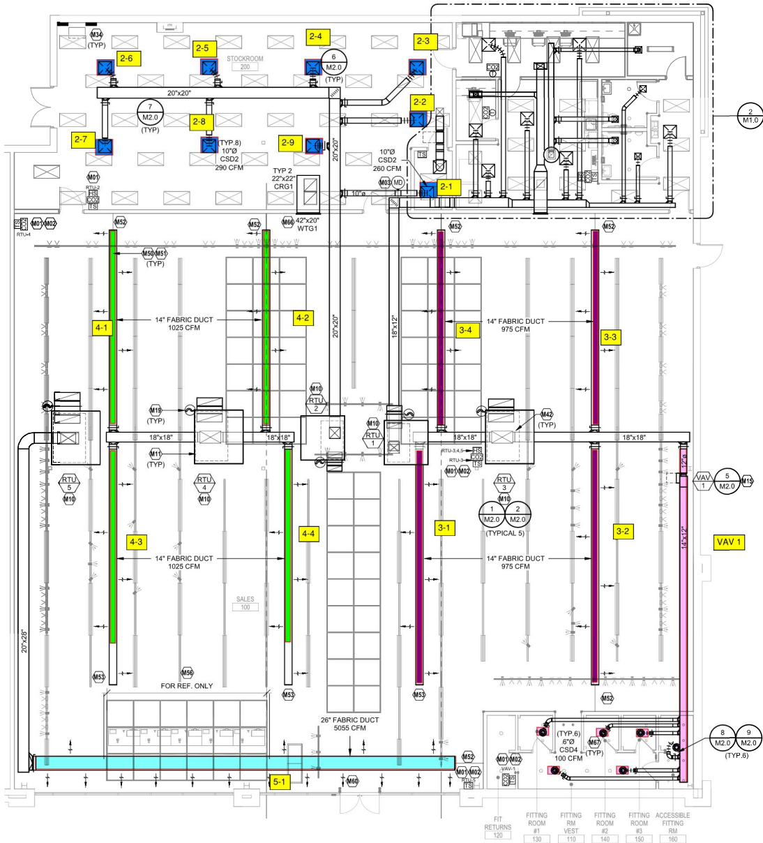
1 HVAC PLAN 1/8" = 1'-0"
