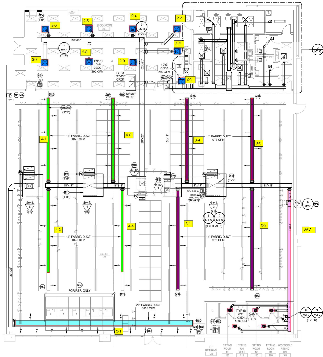
① HVAC PLAN 1/8" = 1'-0"
