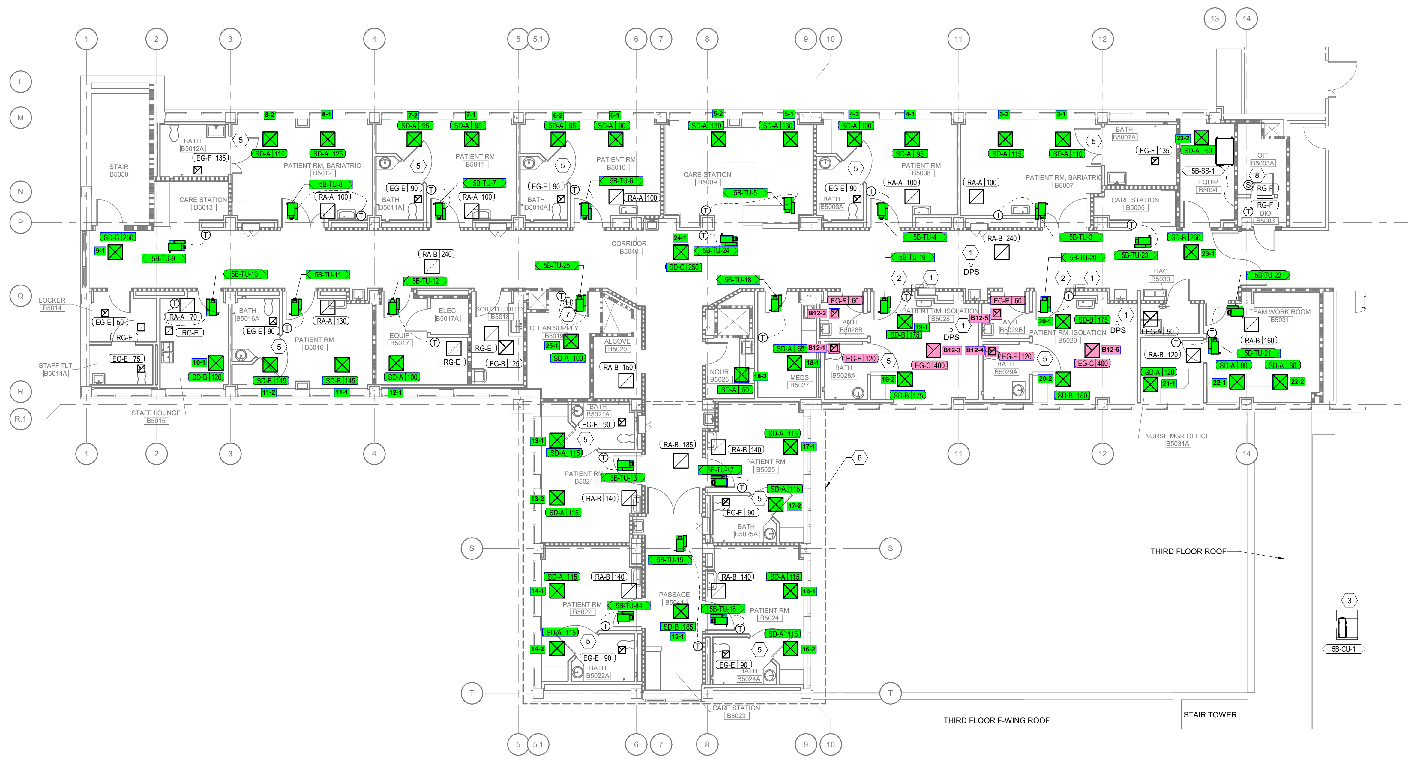
1 FIFTH FLOOR HVAC PLAN Scale: 1/8" = 1'-0"
