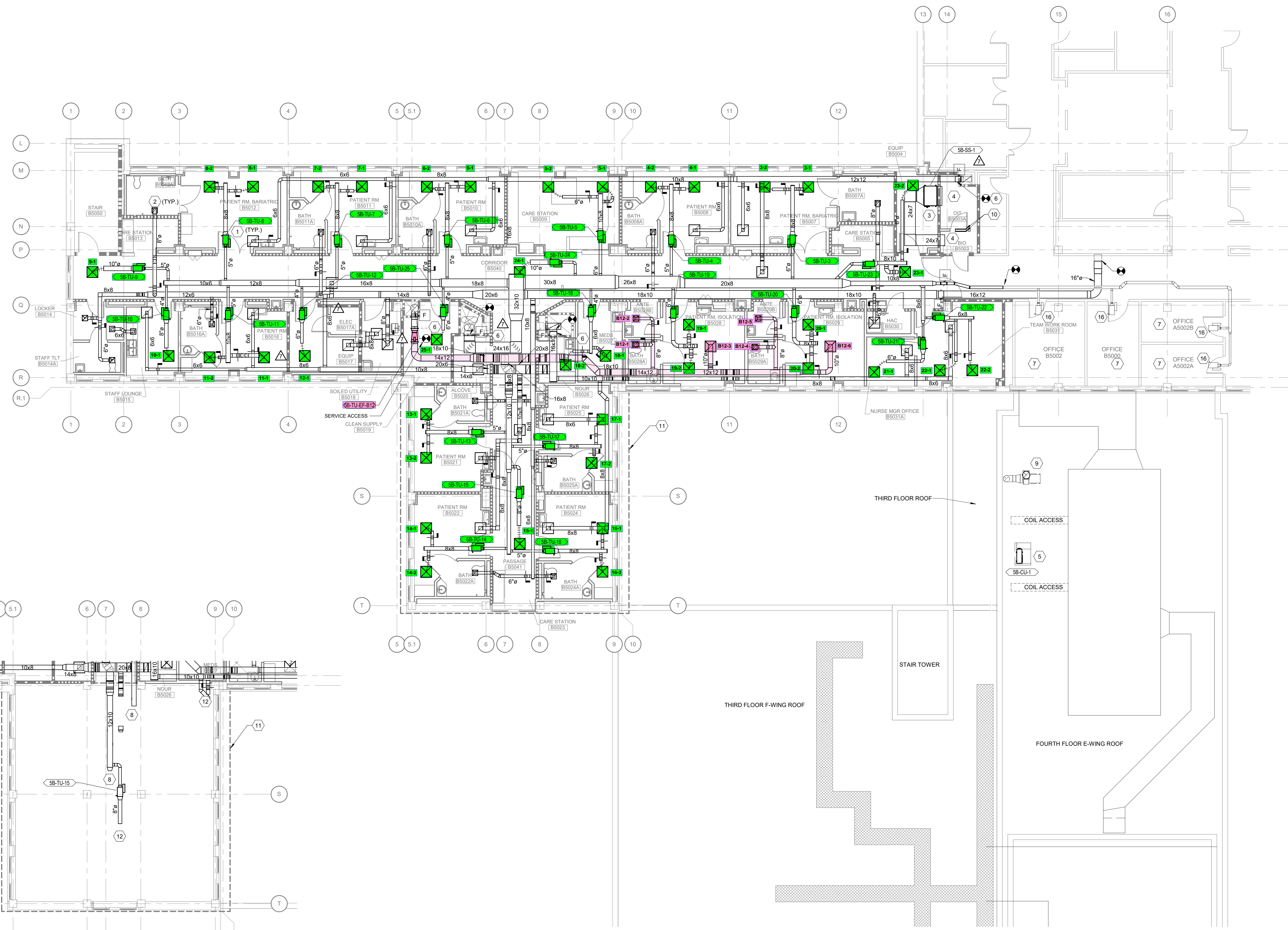
1 FIFTH FLOOR HVAC PLAN Scale: 1/8" = 1'-0"
