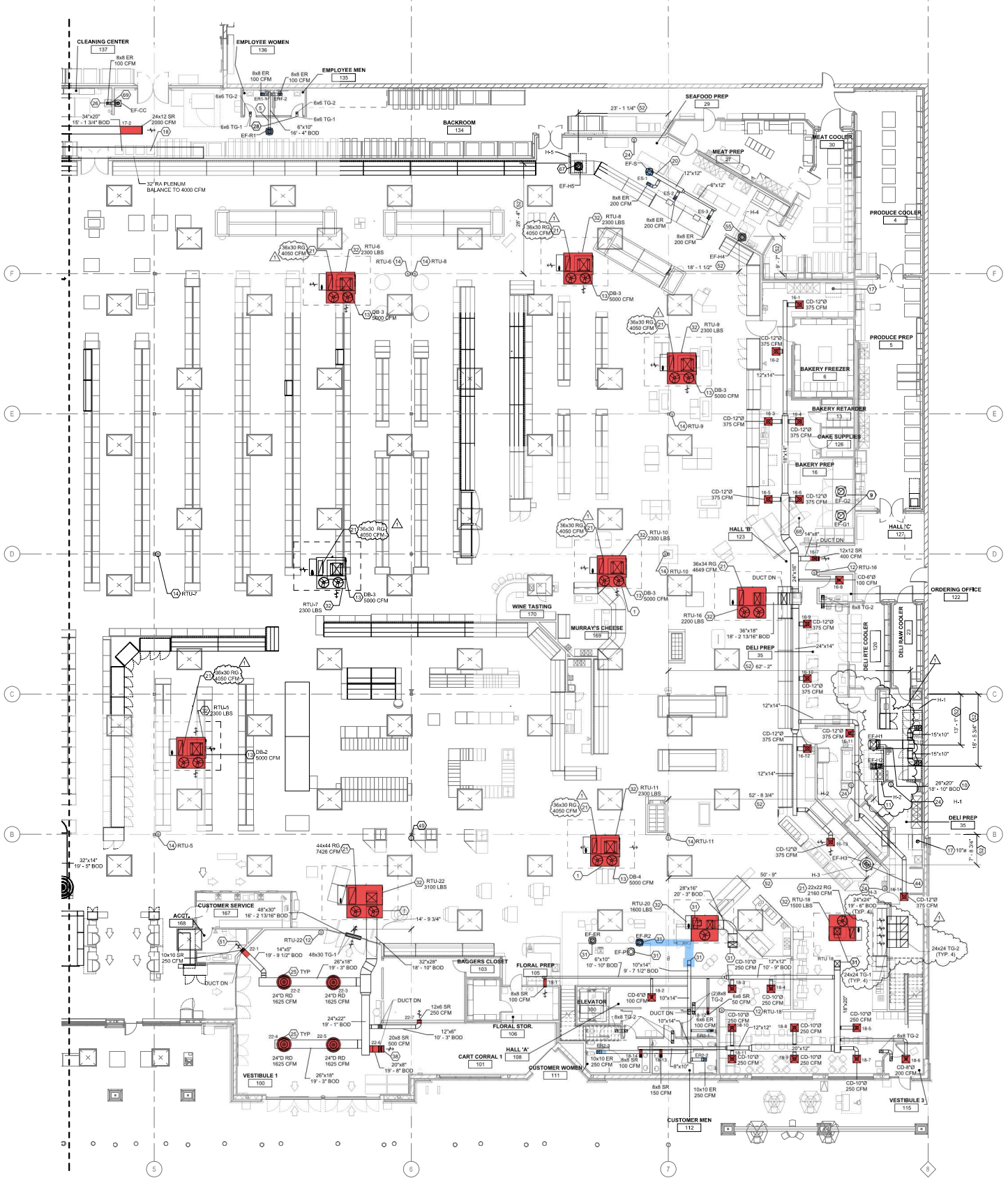
1 HVAC FLOOR PLAN - SOUTH M1.19 SCALE: 3/32" = 1'-0"
