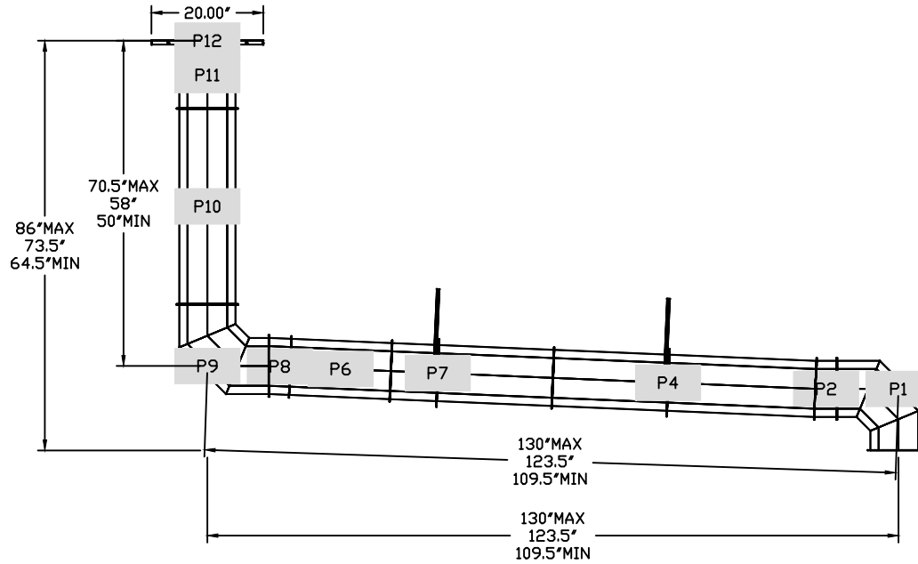
DUCTWORK #2 FRONT VIEW DR2-WILDBERRY
