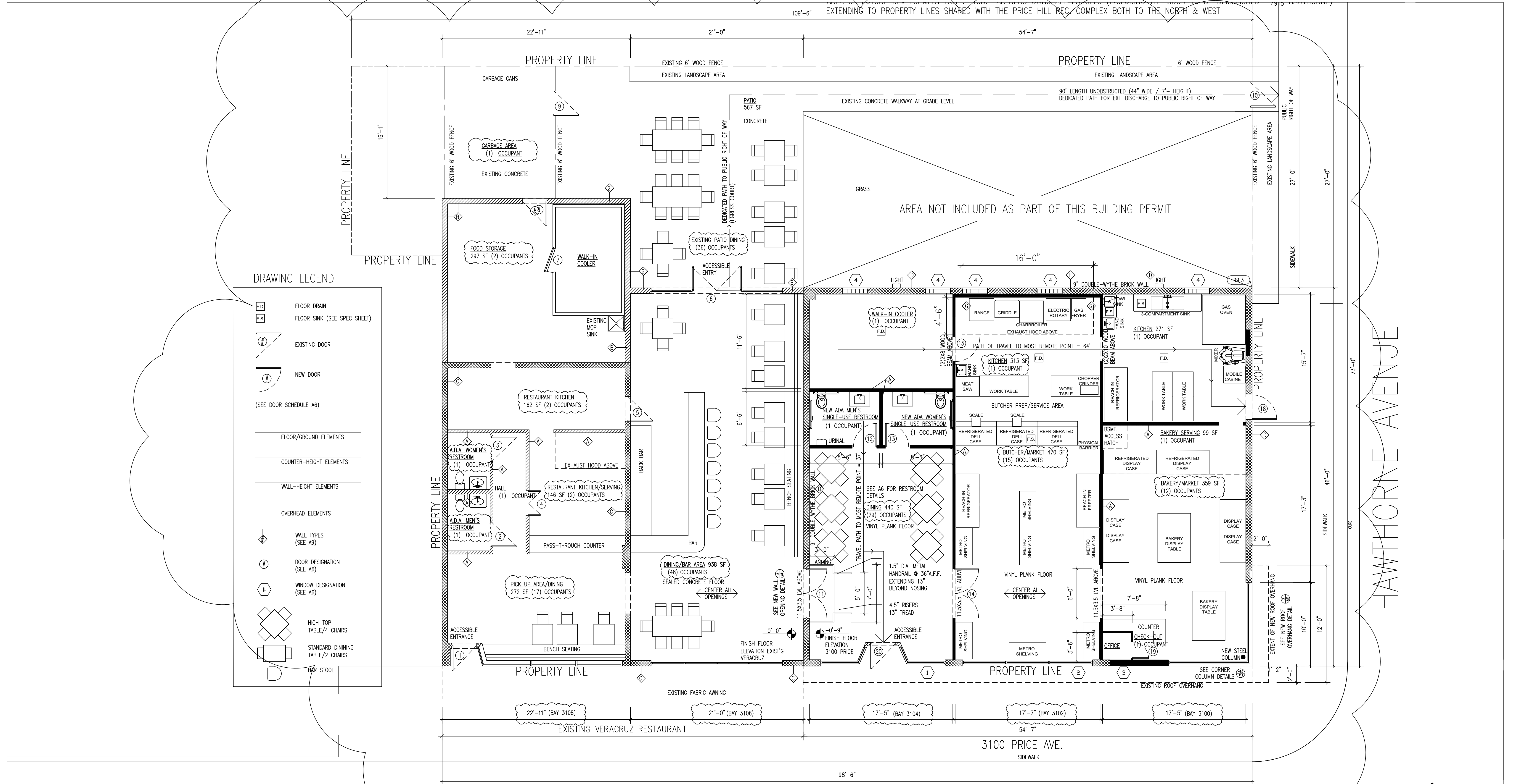
1 PROPOSED FIRST FLOOR PLAN 3/16" = 1'-0"
