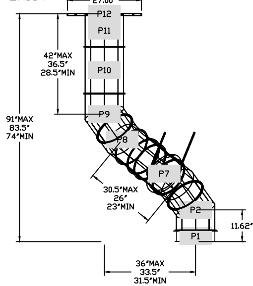
DUCTWORK #1 FRONT VIEW DR4-EXIST
