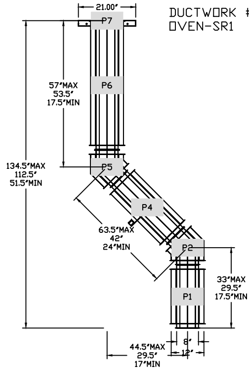
DUCTWORK #1 FRONT VIEW OVEN-SR1
