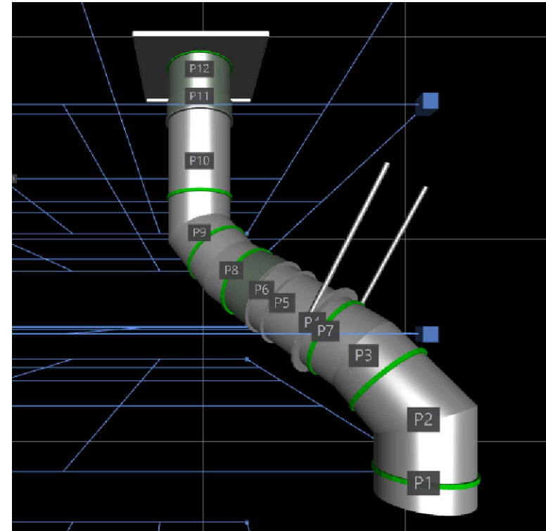
DUCTWORK #1 SE VIEW DR4-EXIST
