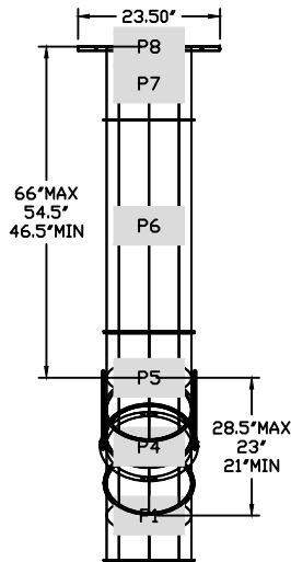
DUCTWORK #3 SIDE VIEW DR-5 GREASE
