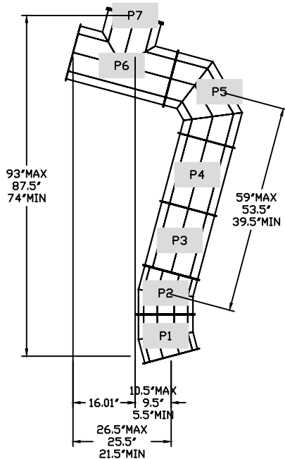
DUCTWORK #3 FRONT VIEW MISC
