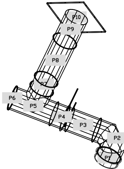
DUCTWORK #2 SE VIEW DR5-EXIST
