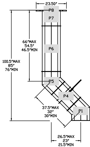
DUCTWORK #2 FRONT VIEW DR-2 GREASE
