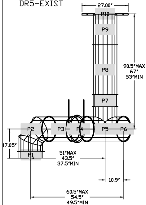
DUCTWORK #2 SIDE VIEW DR5-EXIST
