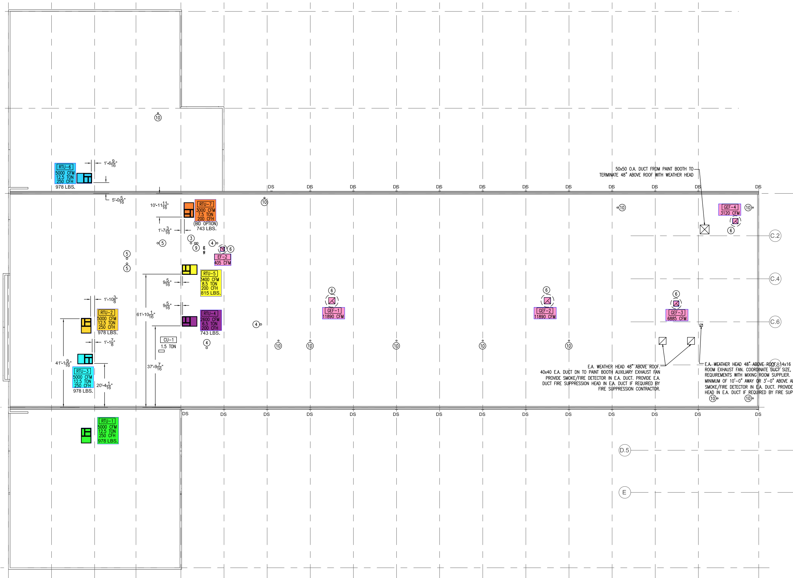
1 MECHANICAL ROOF PLAN M103 Scale: 1/16" = 1'-0"
