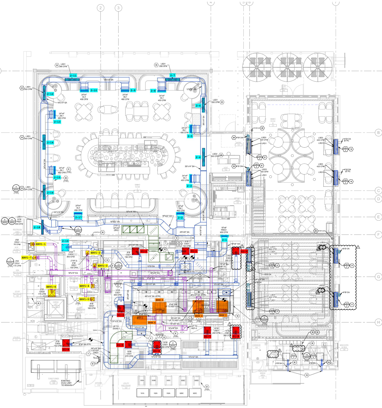
MECHANICAL FIRST FLOOR PLAN 1/4" = 1'-0"
