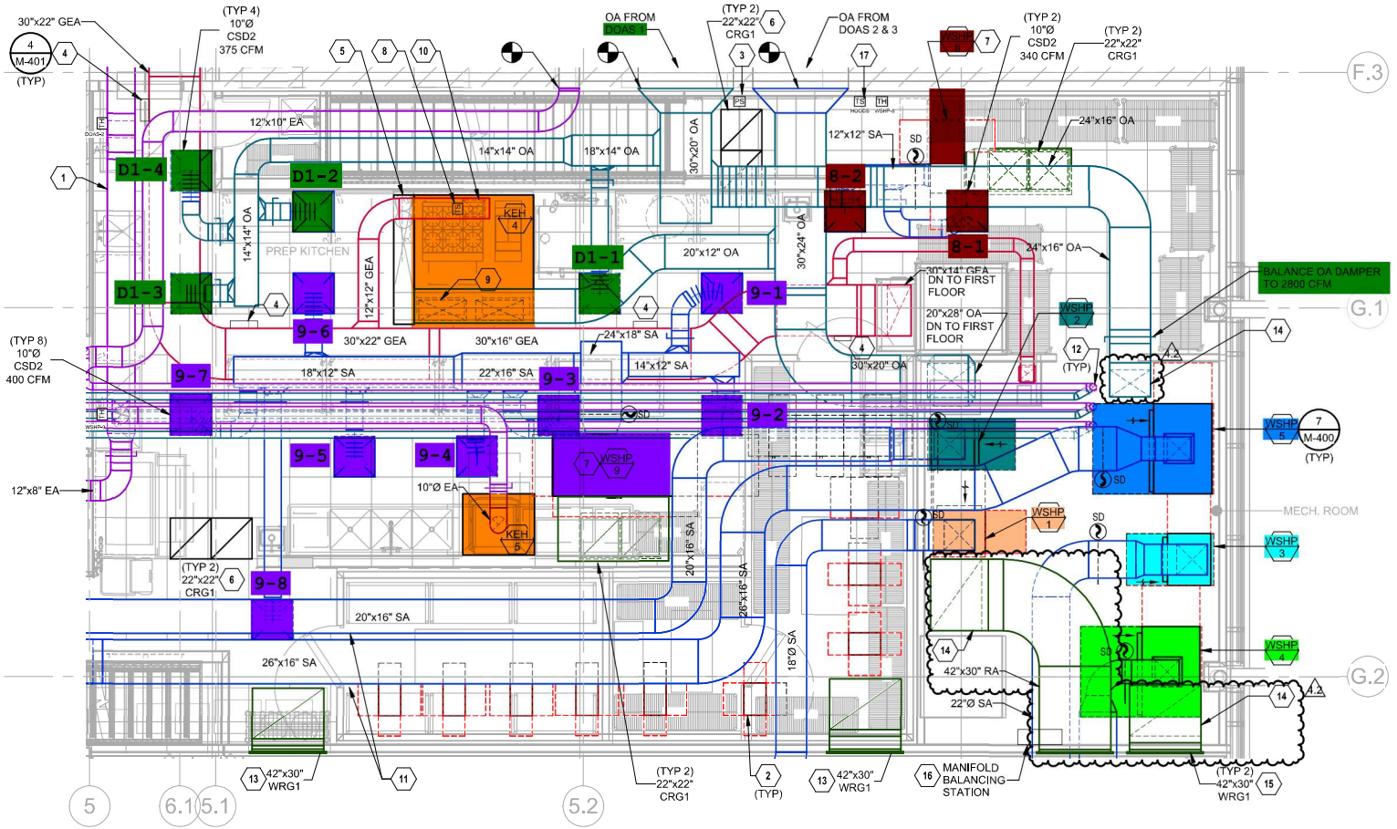
1 ENLARGED MEZZANINE PAGE 1/4" = 1'-0"
