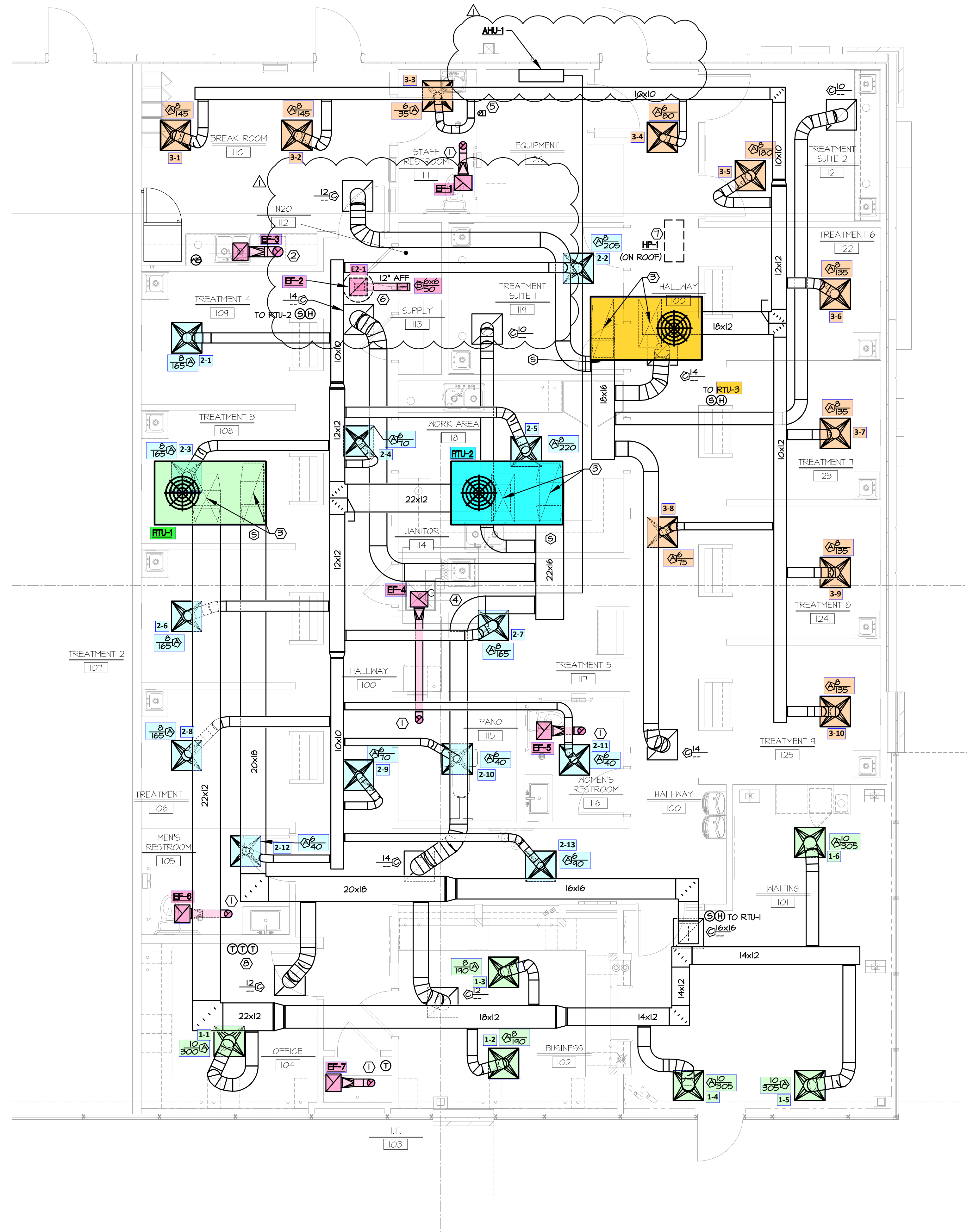
1 FLOOR PLAN - MECHANICAL M101 SCALE: 1/4" = 1'-0"
