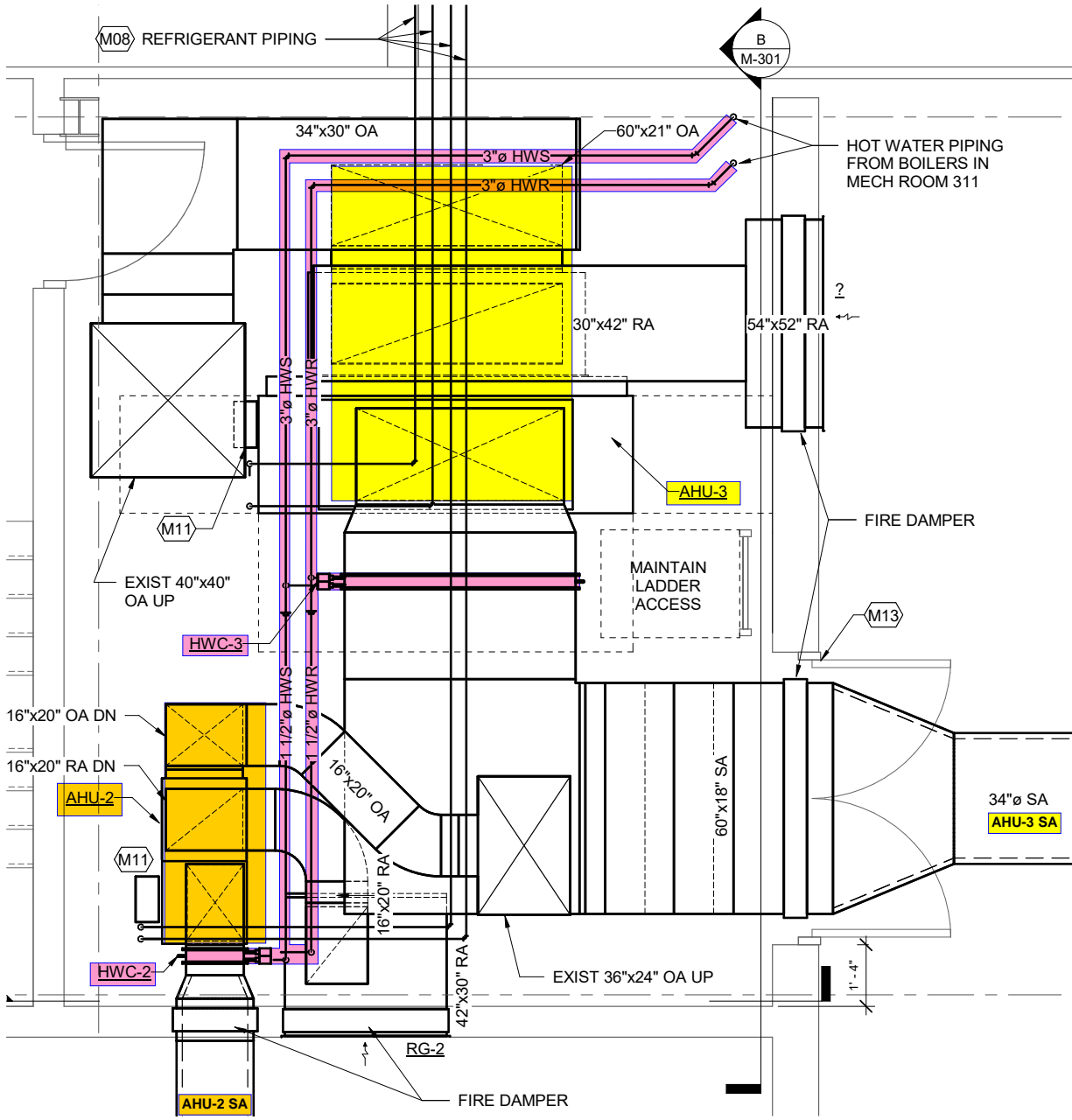
01 AUX GYM MECHANICAL ROOM FLOOR PLAN M-301
