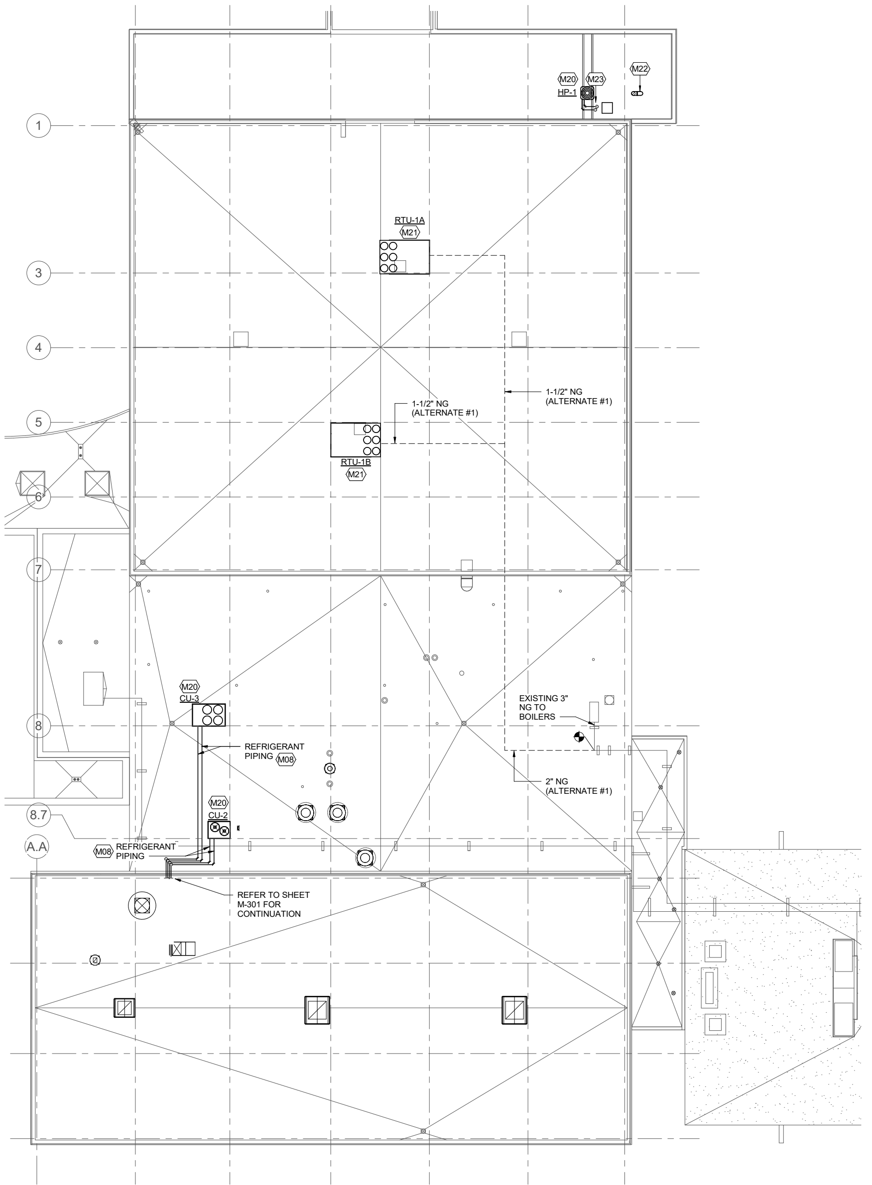
1 BUILDING C - ROOF OVERALL PLAN M-102 3/32" = 1'-0"
