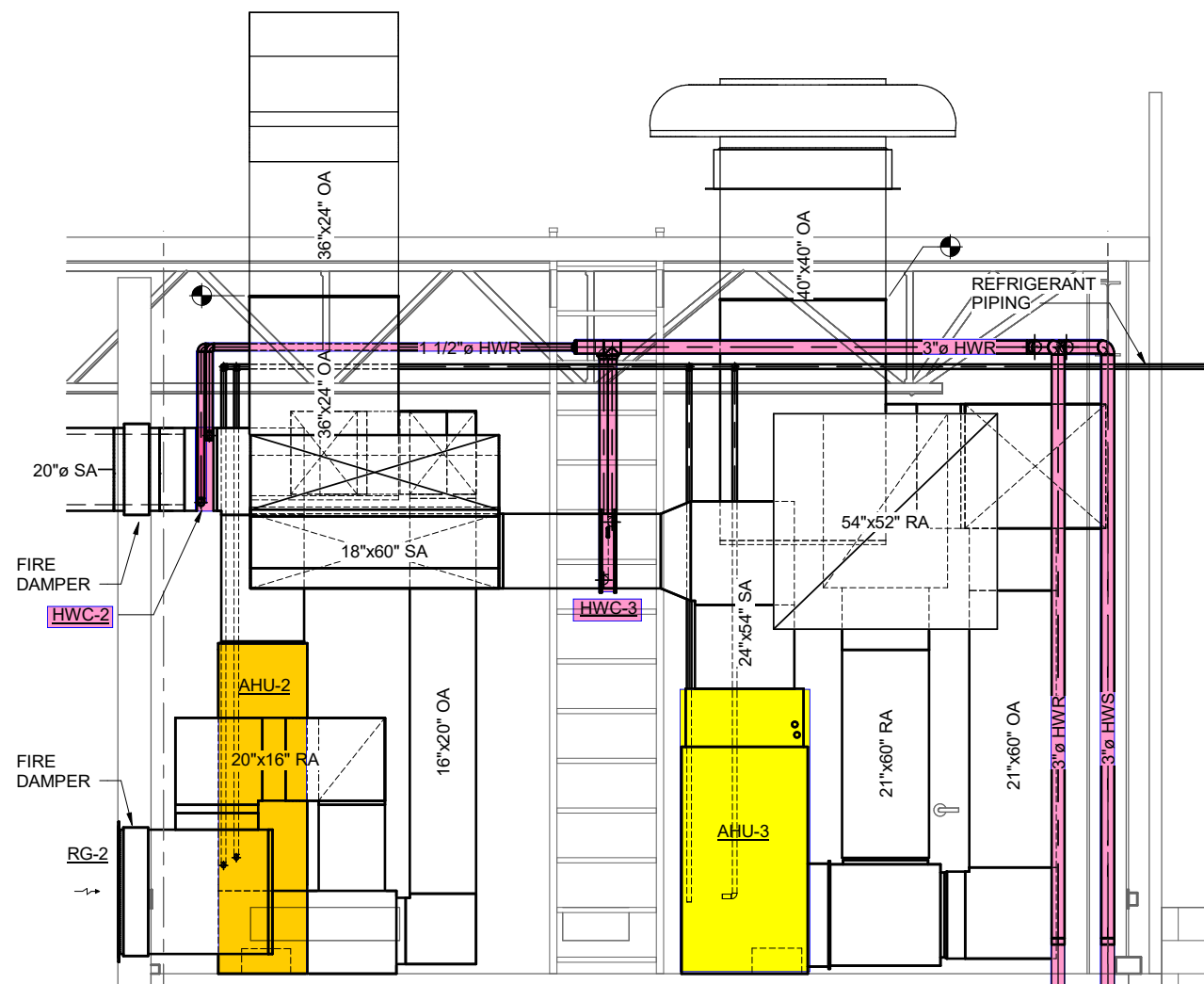
B MECHANICAL ROOM SECTION B M-301
