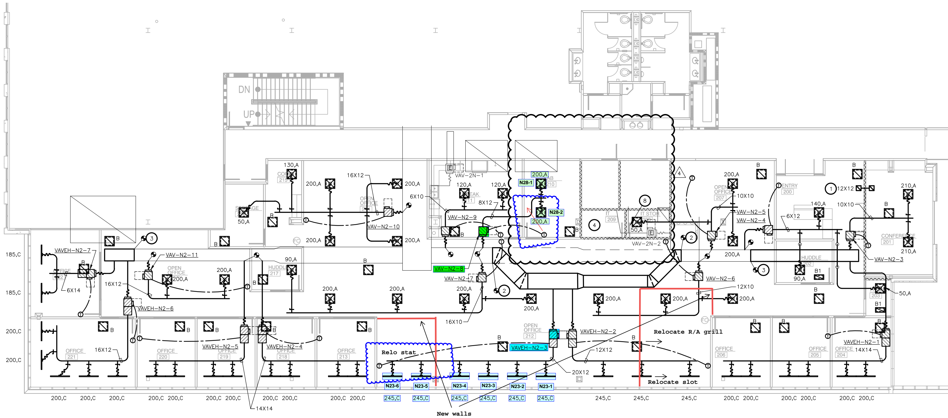
1 LEVEL 02 MECHANICAL PLAN SCALE: 1/8"=1'-0"
