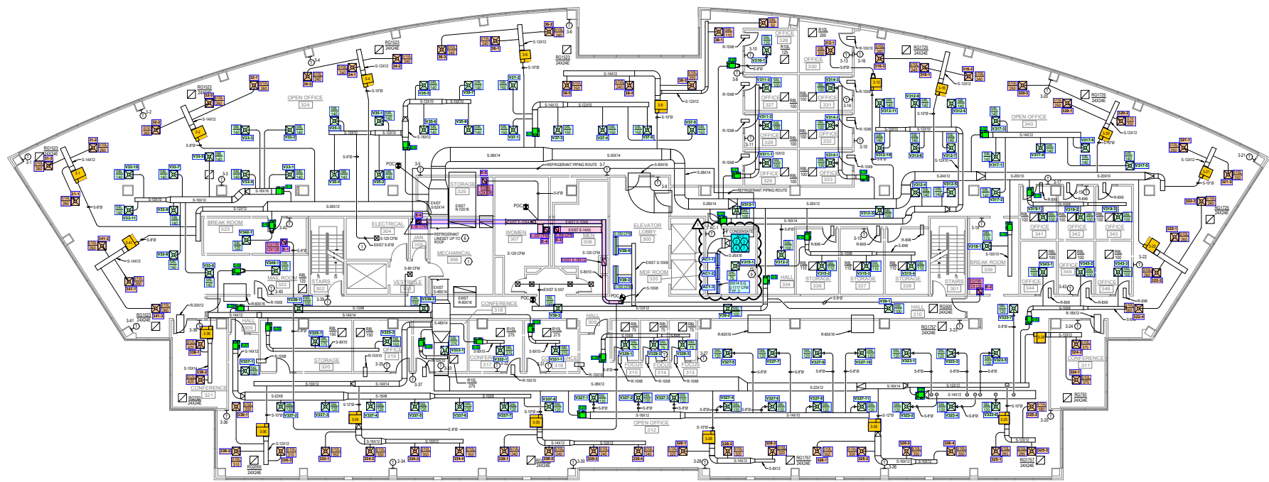
THIRD FLOOR MECHANICAL PLAN SCALE 1/8"=1'-0"
