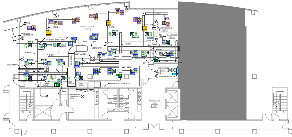
FOURTH FLOOR MECHANICAL PLAN SCALE 1/8"=1'-0"
