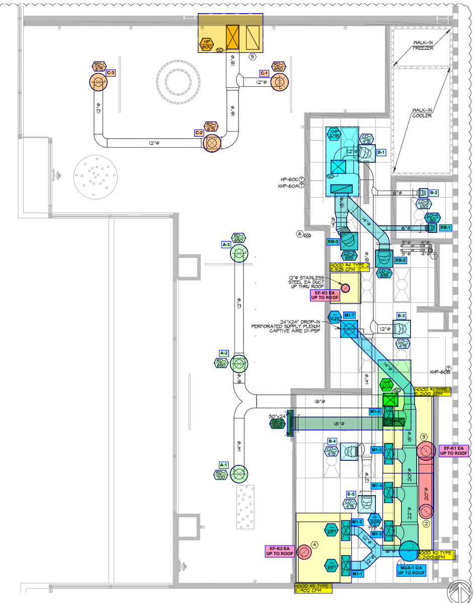
HVAC CEILING PLAN
