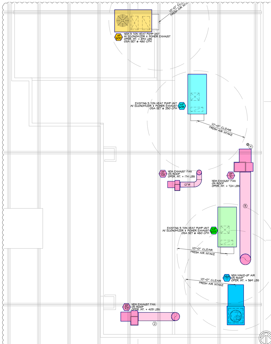
HVAC ROOF PLAN
