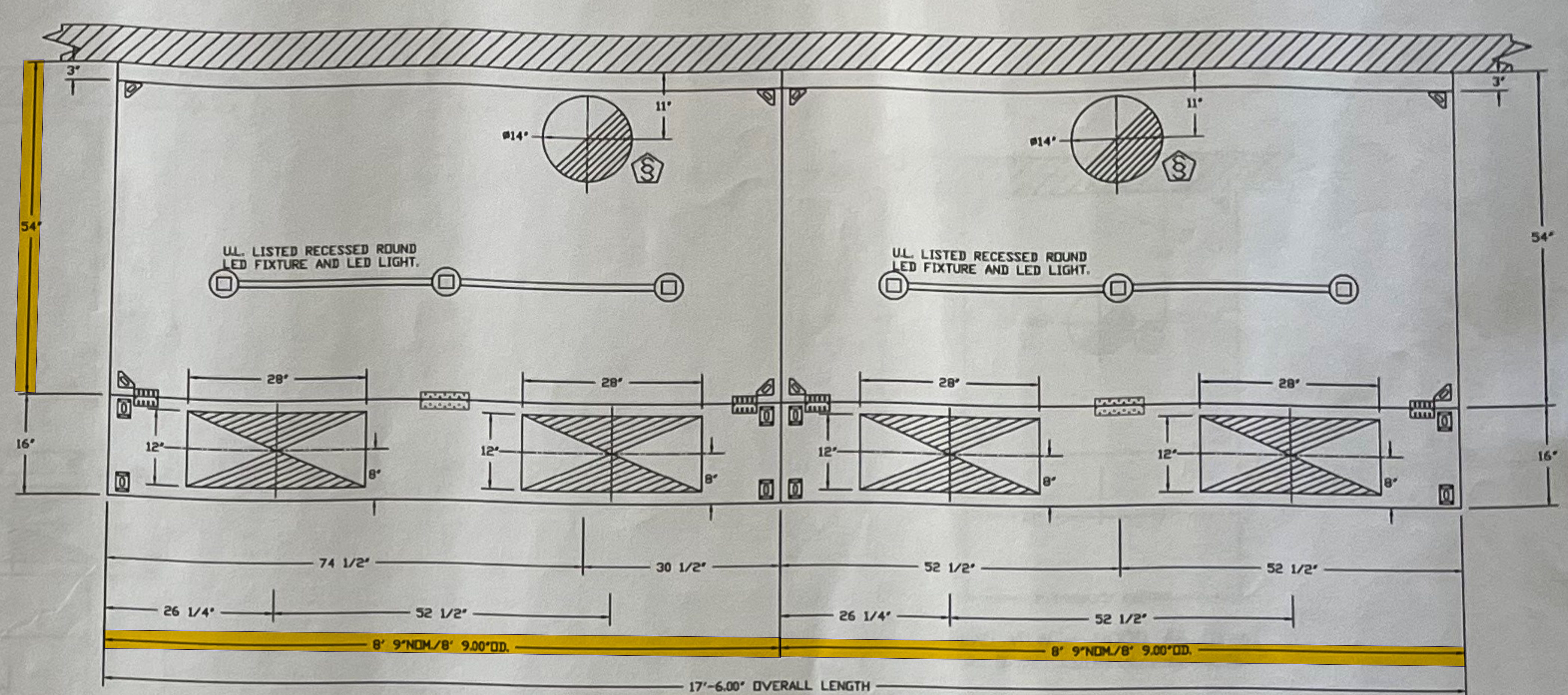
PLAN VIEW - HOOD #1 (15) 8' 9.00" LONG 5424ND-2-PSP-F
