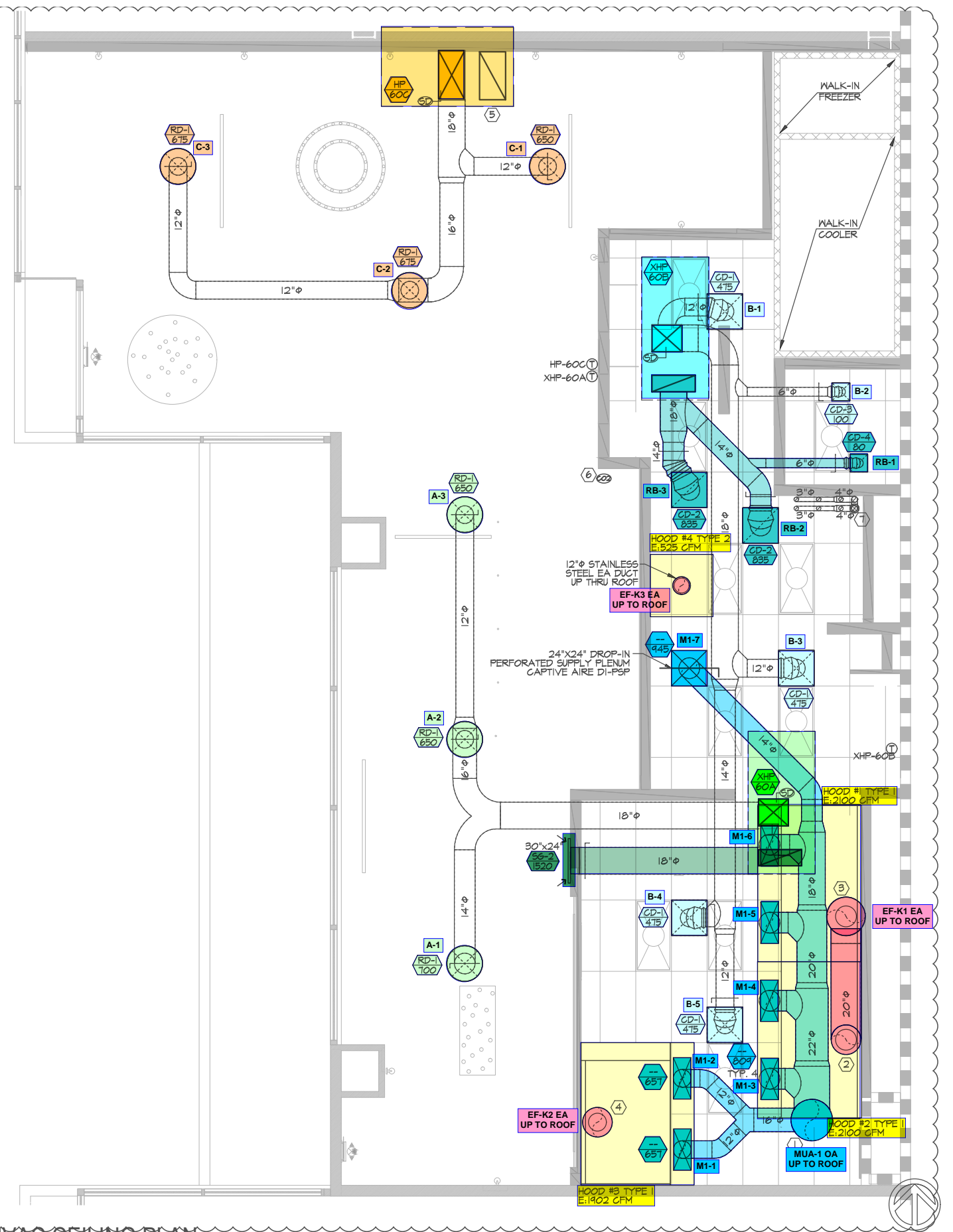
HVAC CEILING PLAN
