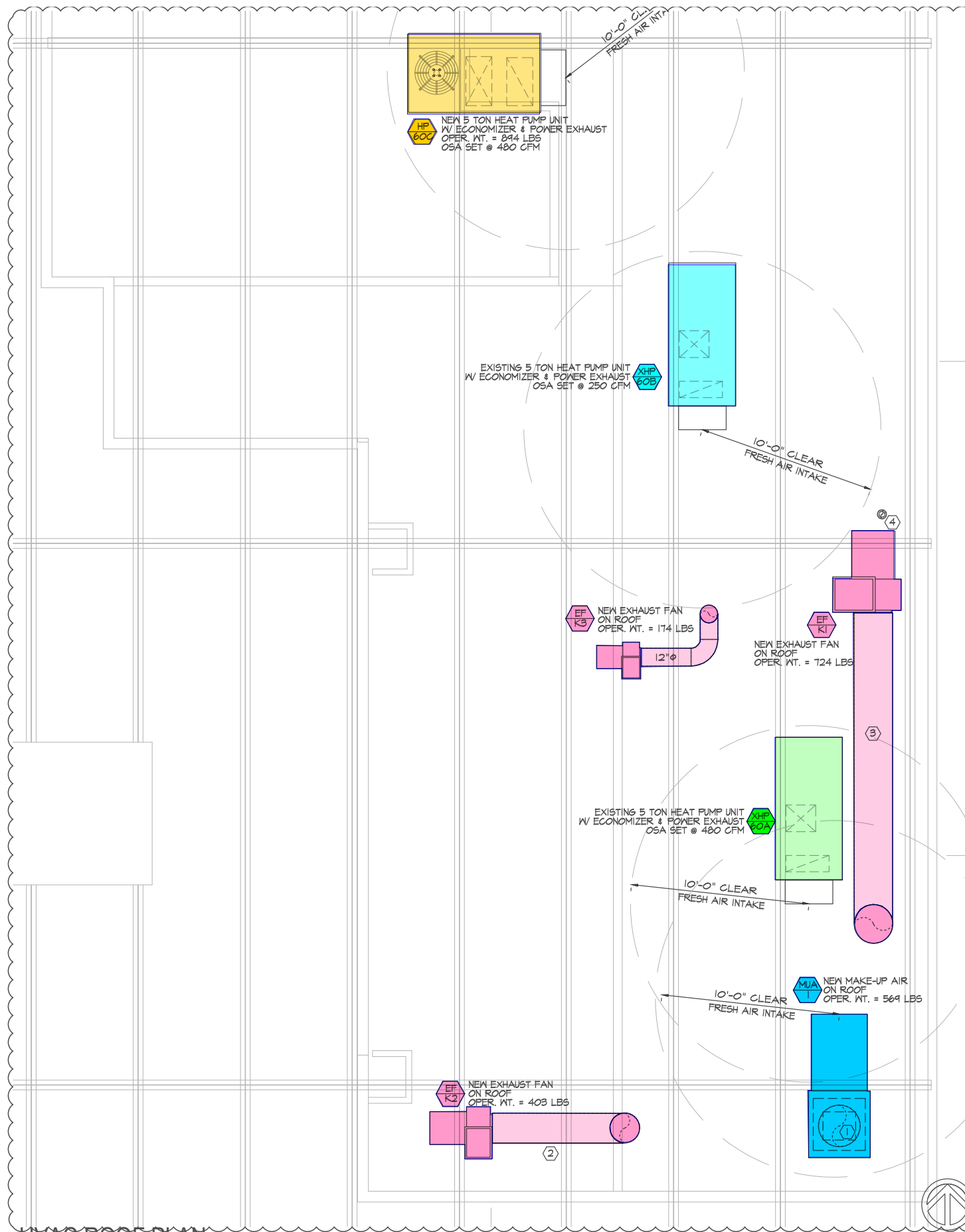
HVAC ROOF PLAN
