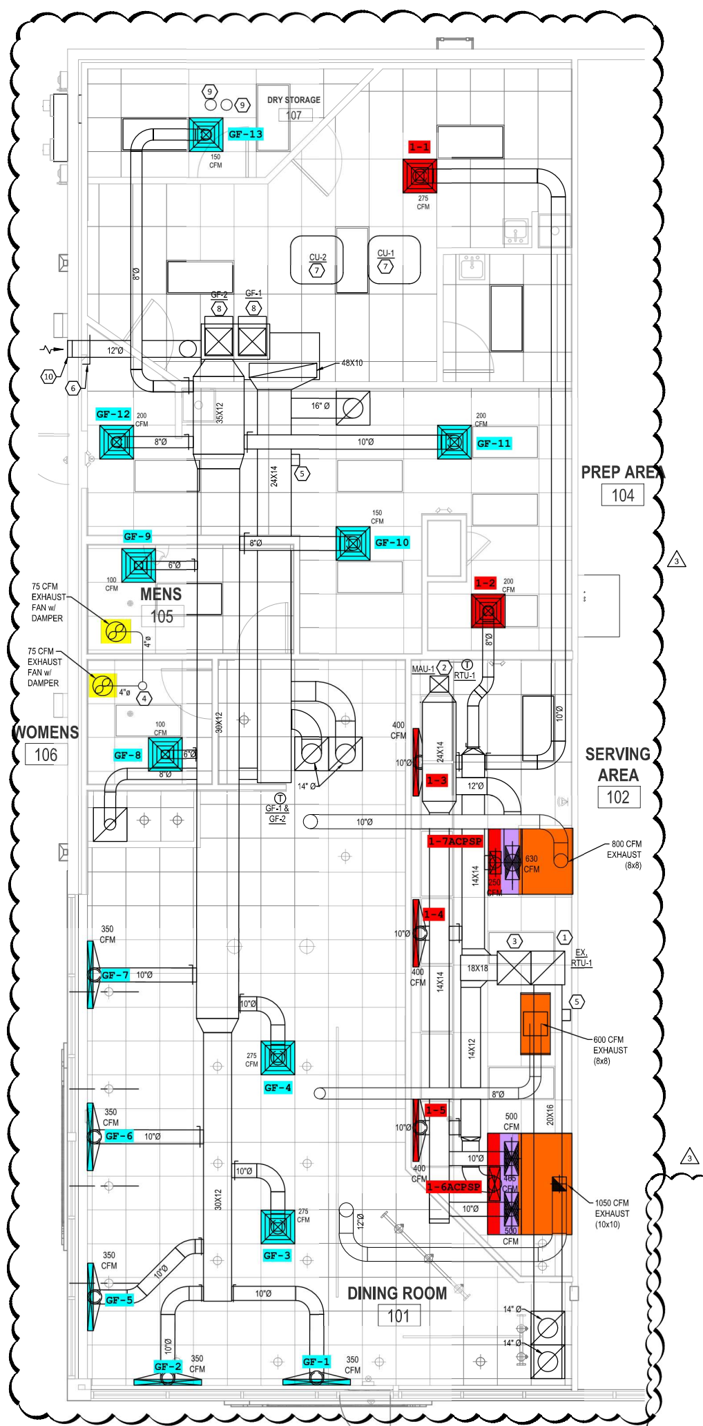
MECHANICAL - FLOOR PLAN
