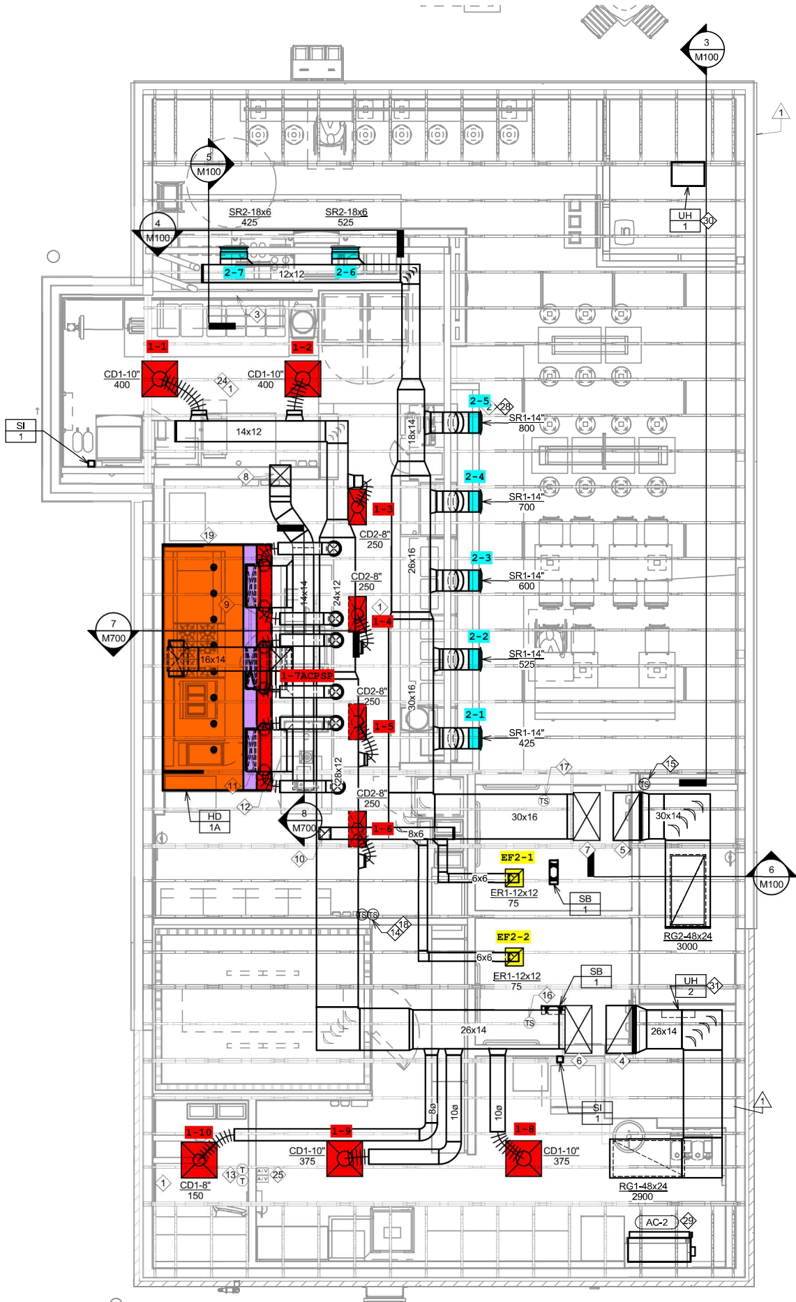
① HVAC FLOOR PLAN 1/4" = 1'-0"
