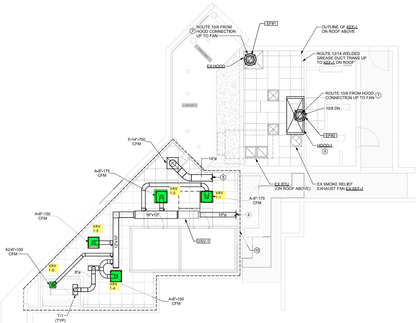
1 MECHANICAL FLOOR PLAN 1/4" = 1'-0"
