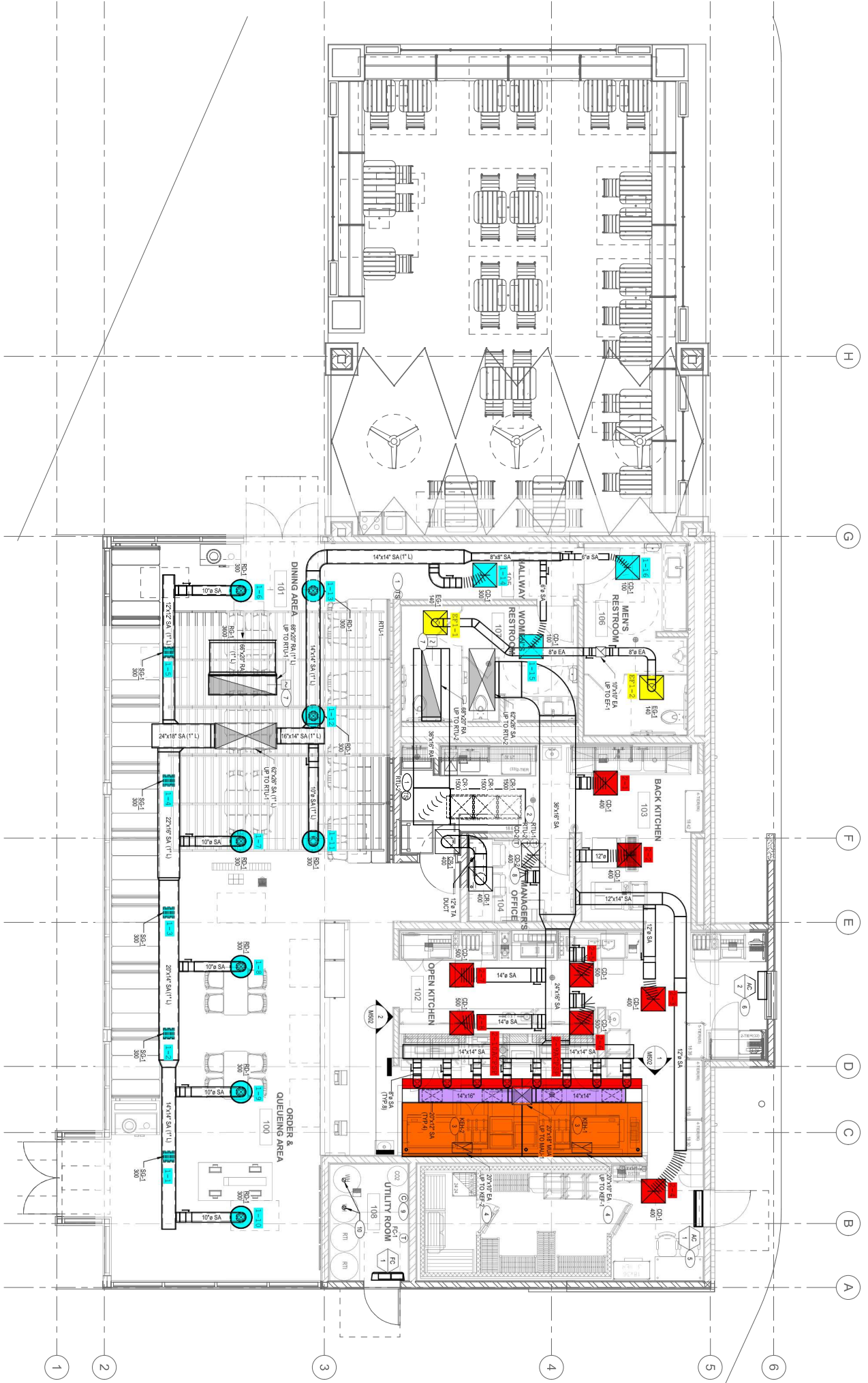
MECHANICAL FLOOR PLAN 1 SCALE: 1/4" = 1'-0"
