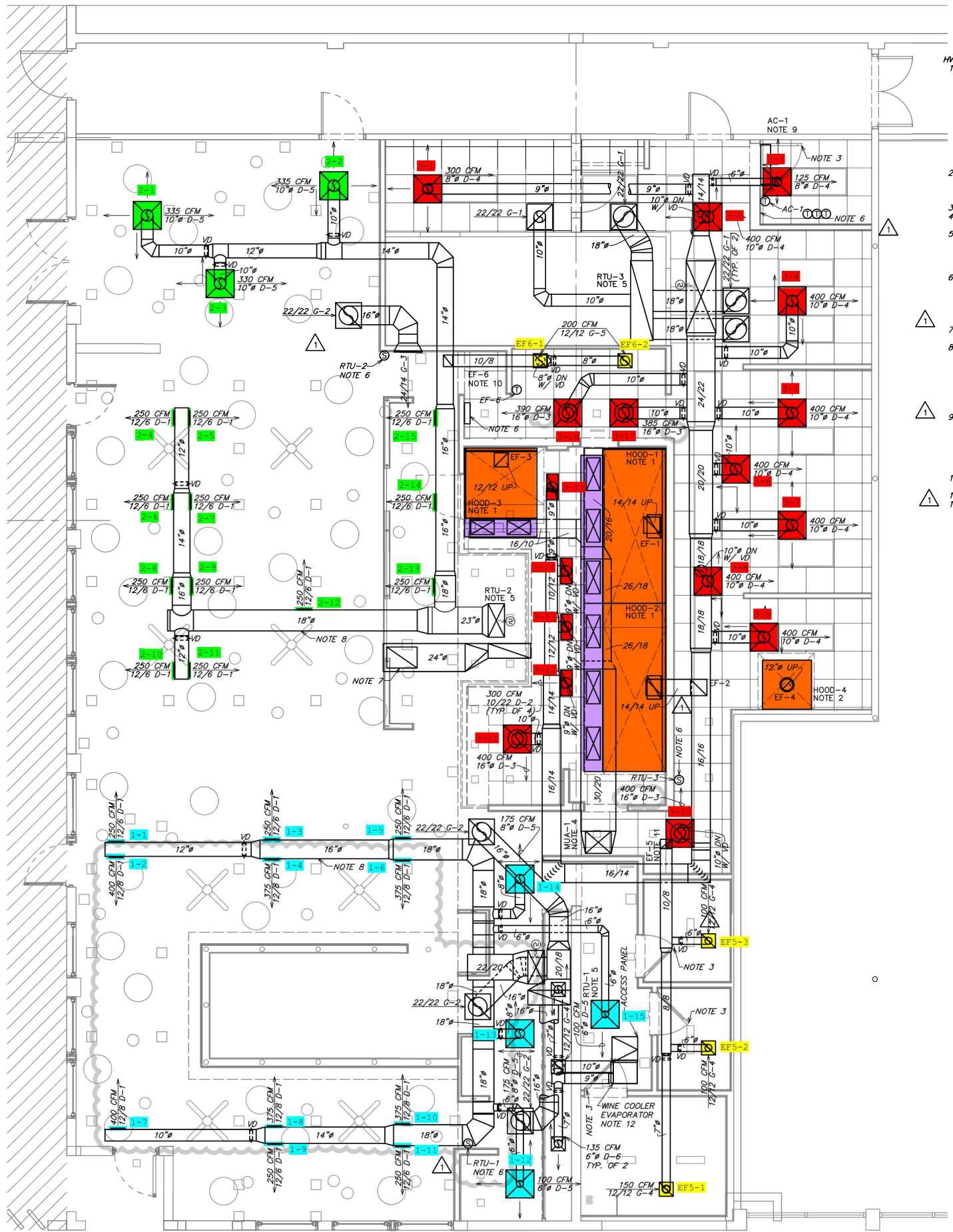
1 MEP ROOF PLAN 1/4" = 1'-0"
