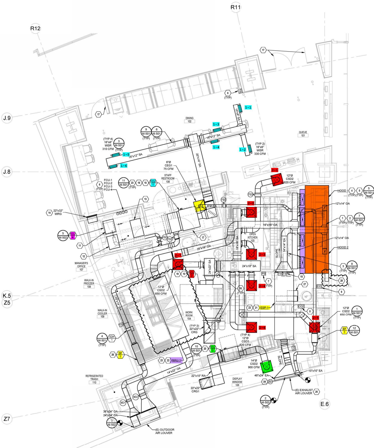
1 MECHANICAL FLOOR PLAN 1/4" = 1'-0"
