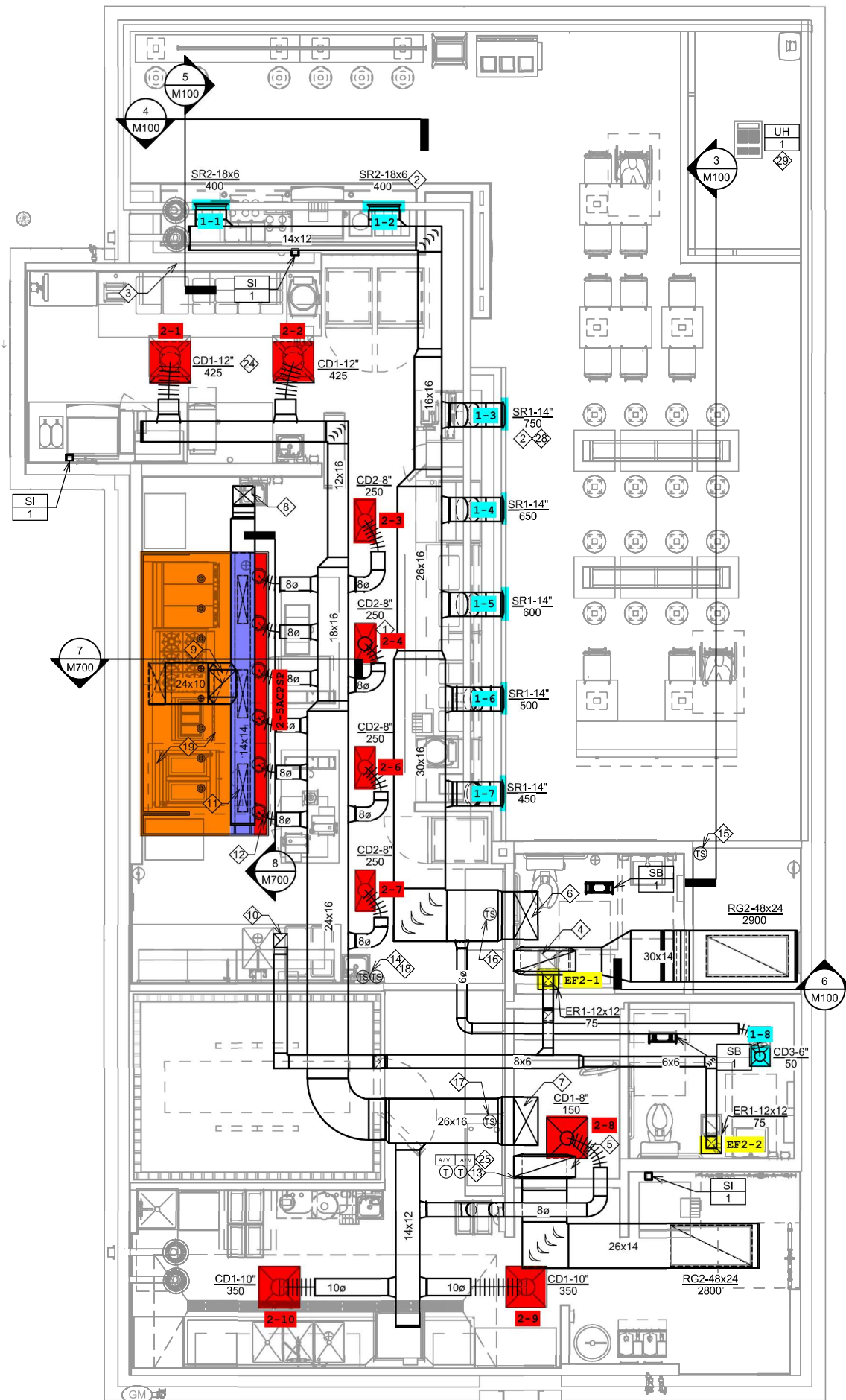
1 HVAC FLOOR PLAN 1/4" = 1'-0"
