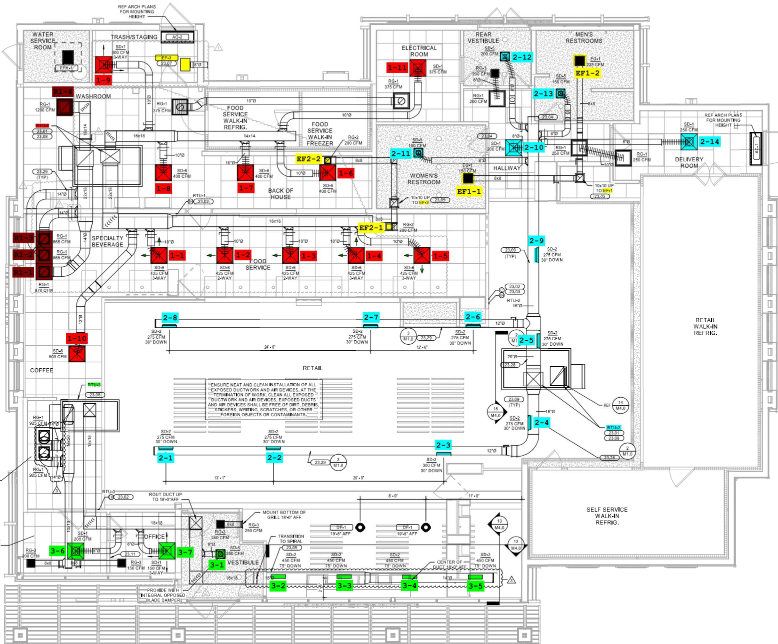
1 HVAC FLOOR PLAN 1/4" = 1'-0"
