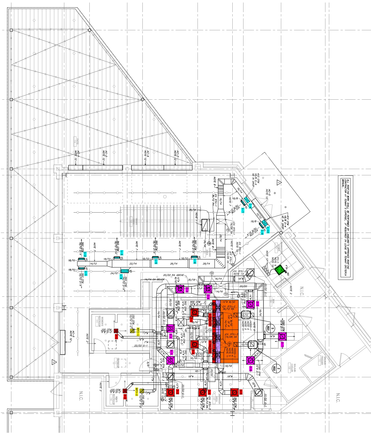
1 MECHANICAL FLOOR PLAN SCALE: 1/4" = 1'-0"
