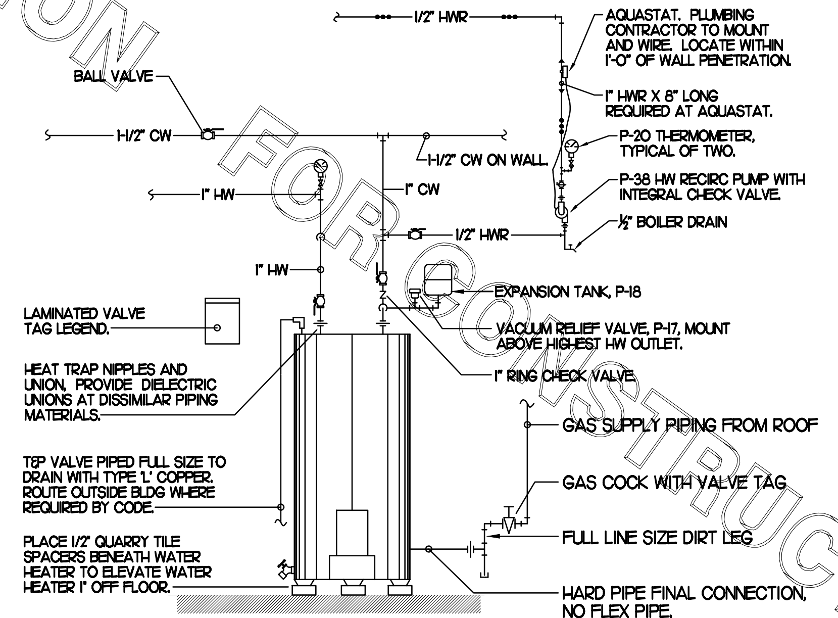
5 WATER HEATER & PIPING DETAIL SCALE: NONE
