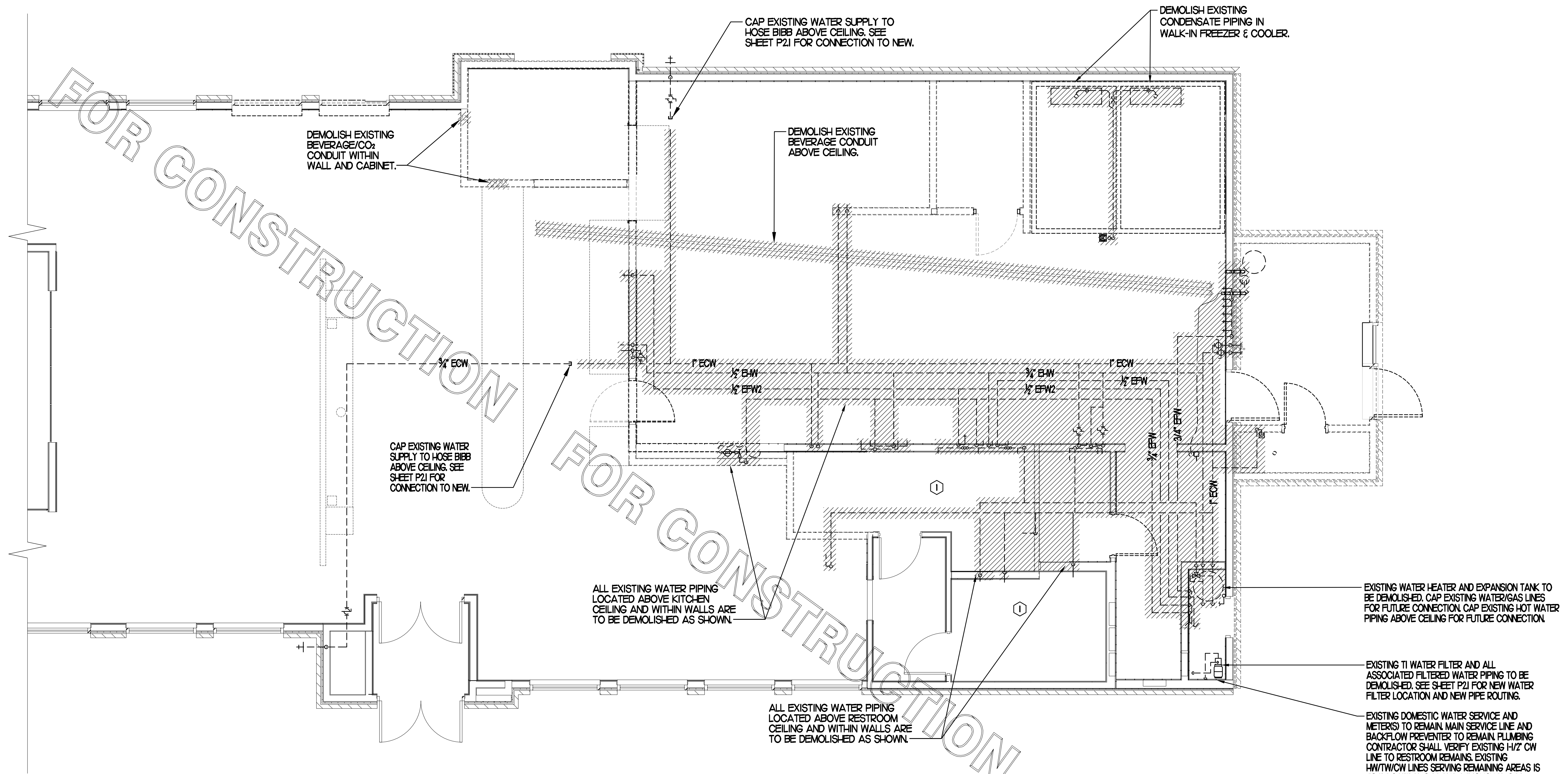
1 ABOVE SLAB PLUMBING DEMOLITION PLAN SCALE: 1/4"=1'-0"
