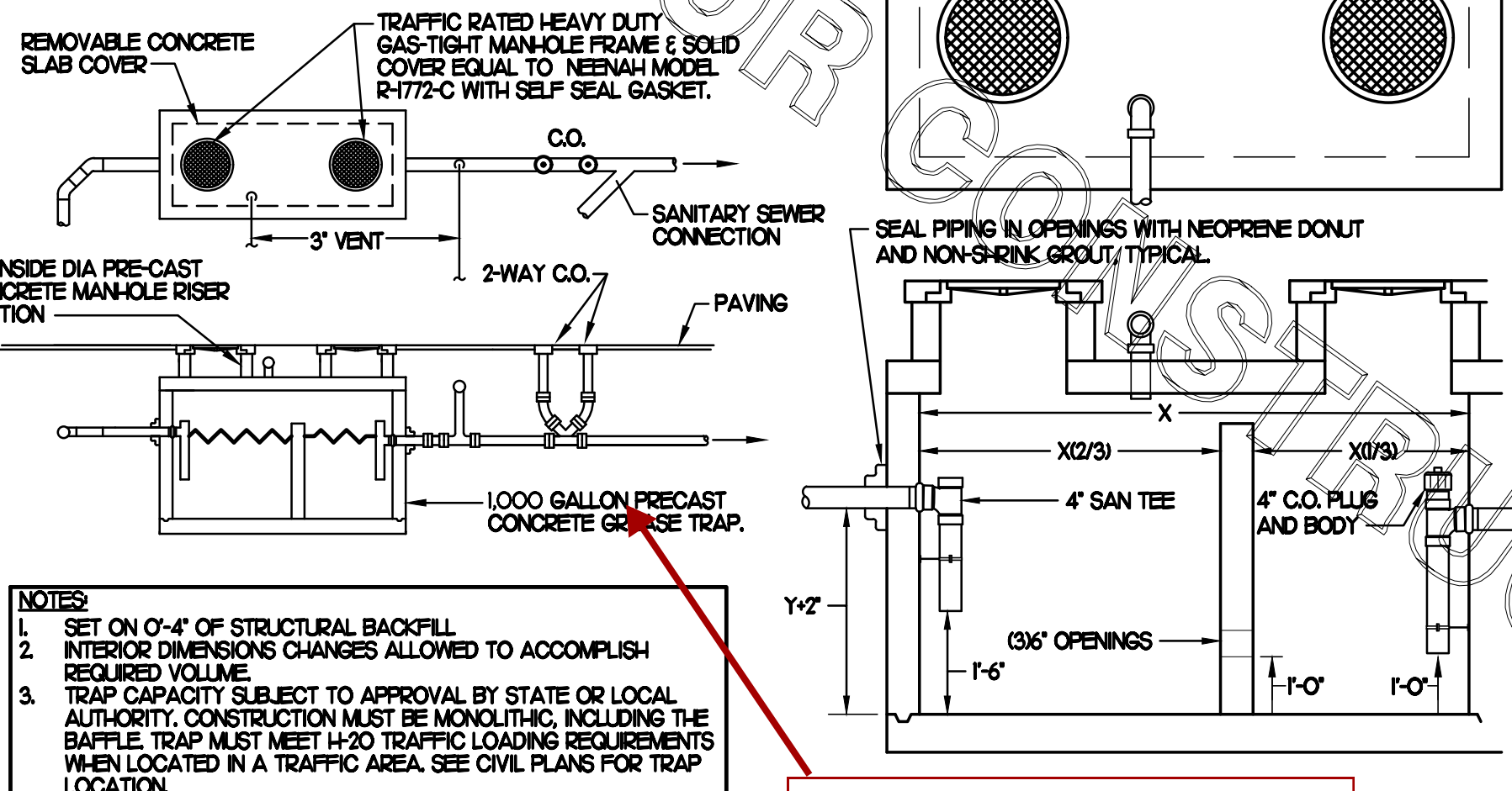
2 GREASE INTERCEPTOR SCALE: NONE
