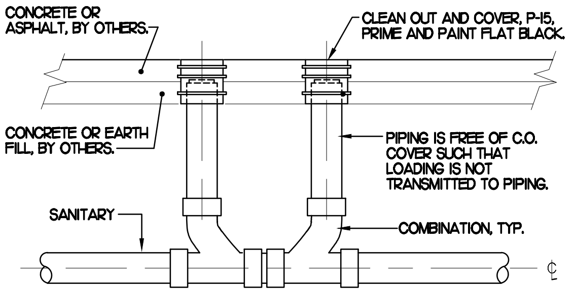
4 SAN. C.O. OUTSIDE BUILDING SCALE: NONE
