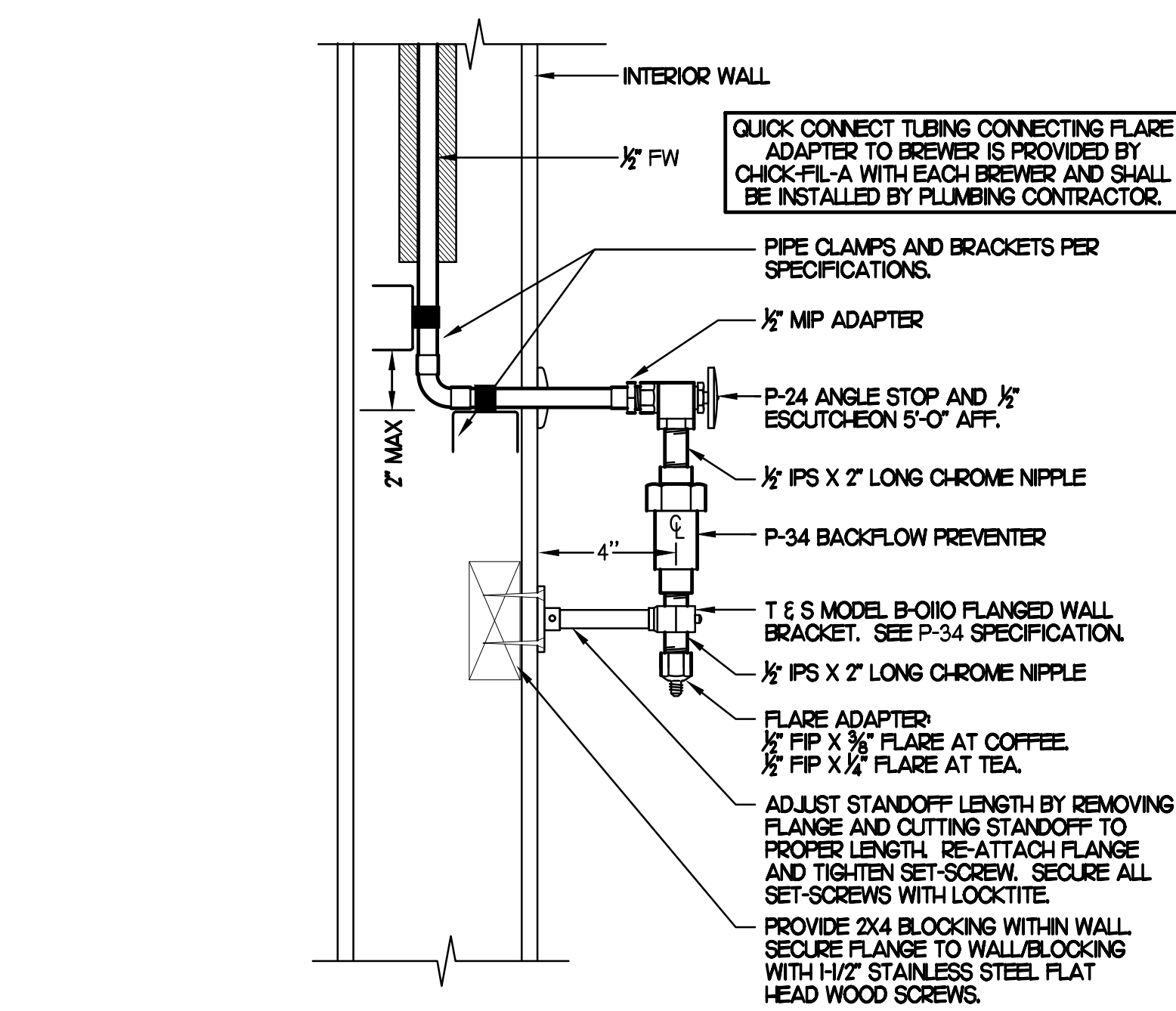
6 COFFEE & TEA BREWER STOP & BFP NO SCALE
