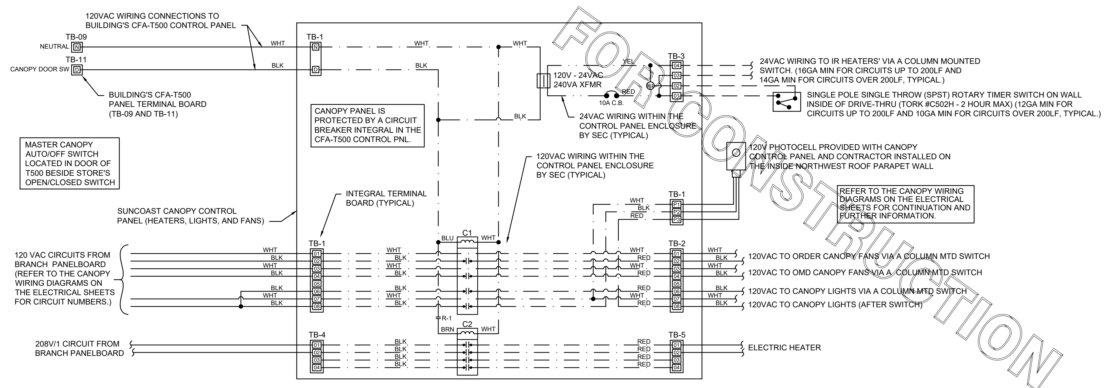
1 SUNCOAST PANEL WIRING DIAGRAM - HEATERS, COOLING FANS NO SCALE CONNECTING WITH A NEW OR REPLACEMENT CFA-T500 CONTROL PANEL
