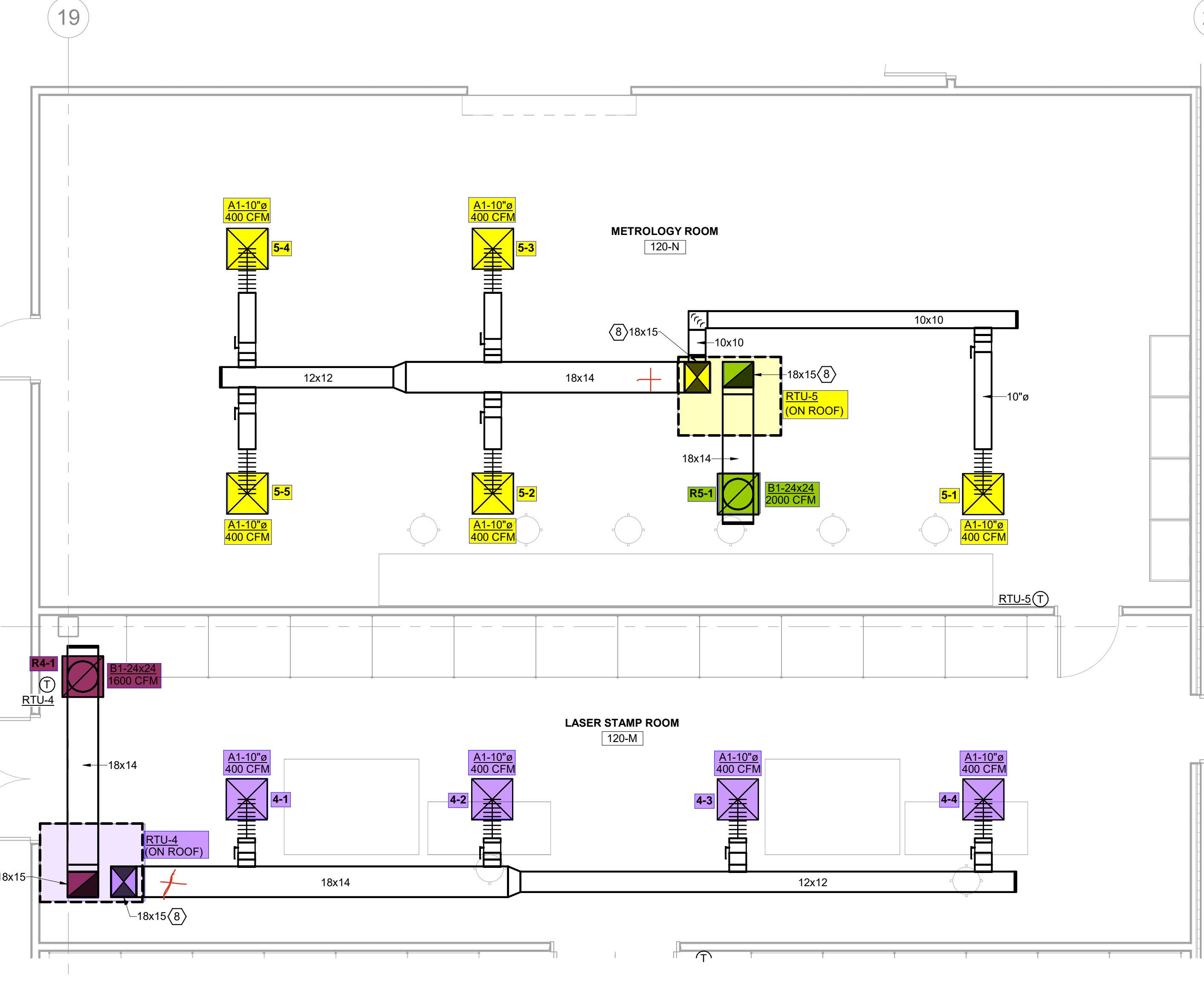
④ ENLARGED HVAC PLAN - NEW WORK 1/4" = 1'-0"
