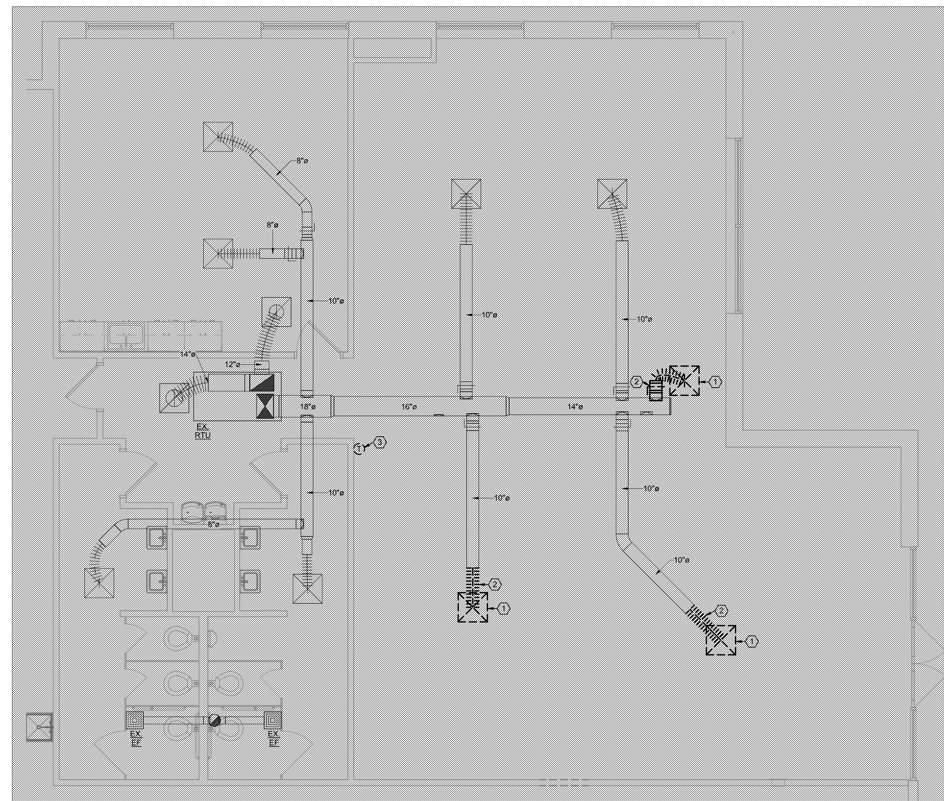
1 ENLARGED HVAC PLAN - DEMOLITION 1/4" = 1'-0"
