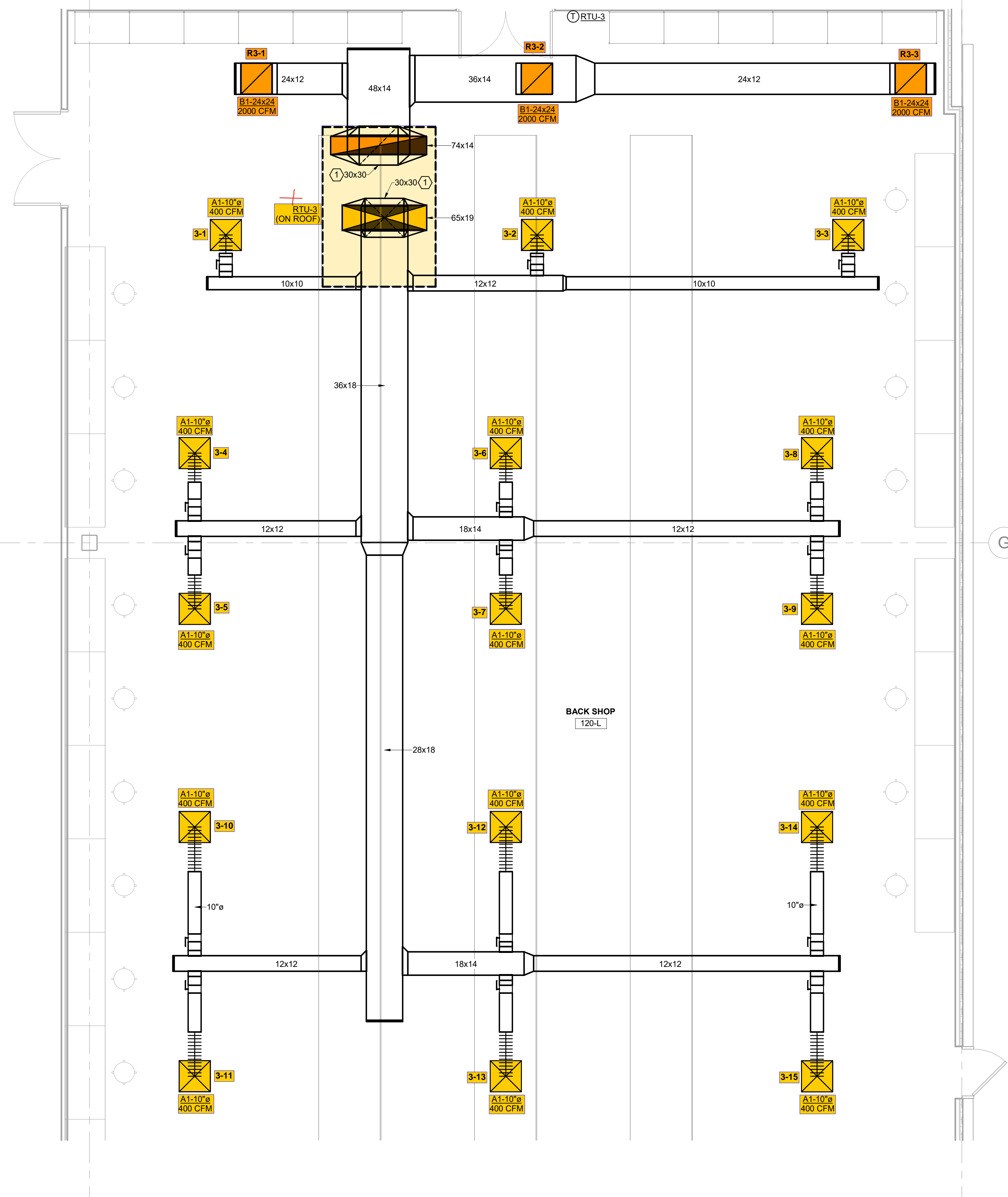
① ENLARGED HVAC PLAN - NEW WORK 1/4" = 1'-0"
