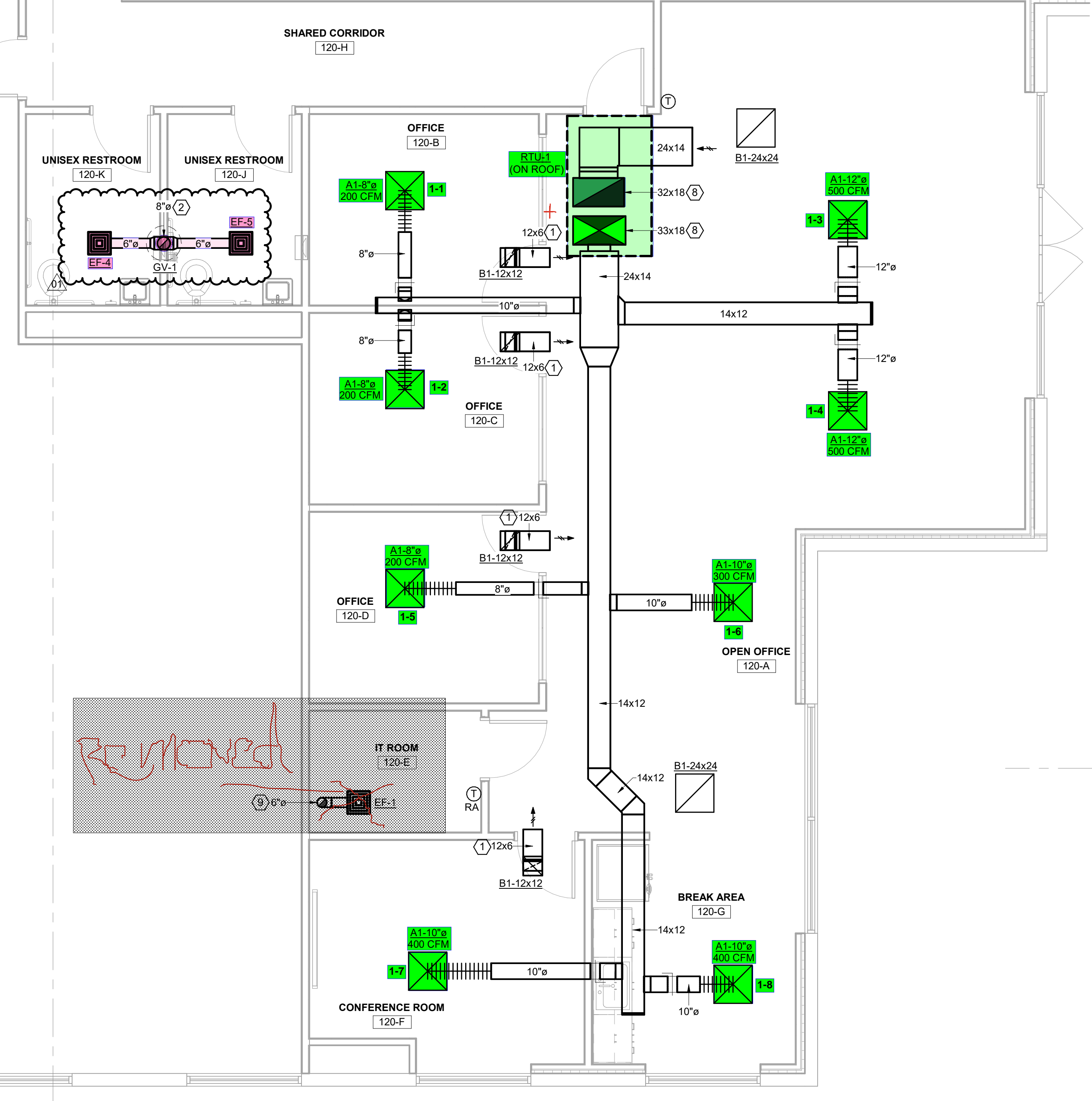
① ENLARGED HVAC PLAN - NEW WORK 1/4" = 1'-0"
