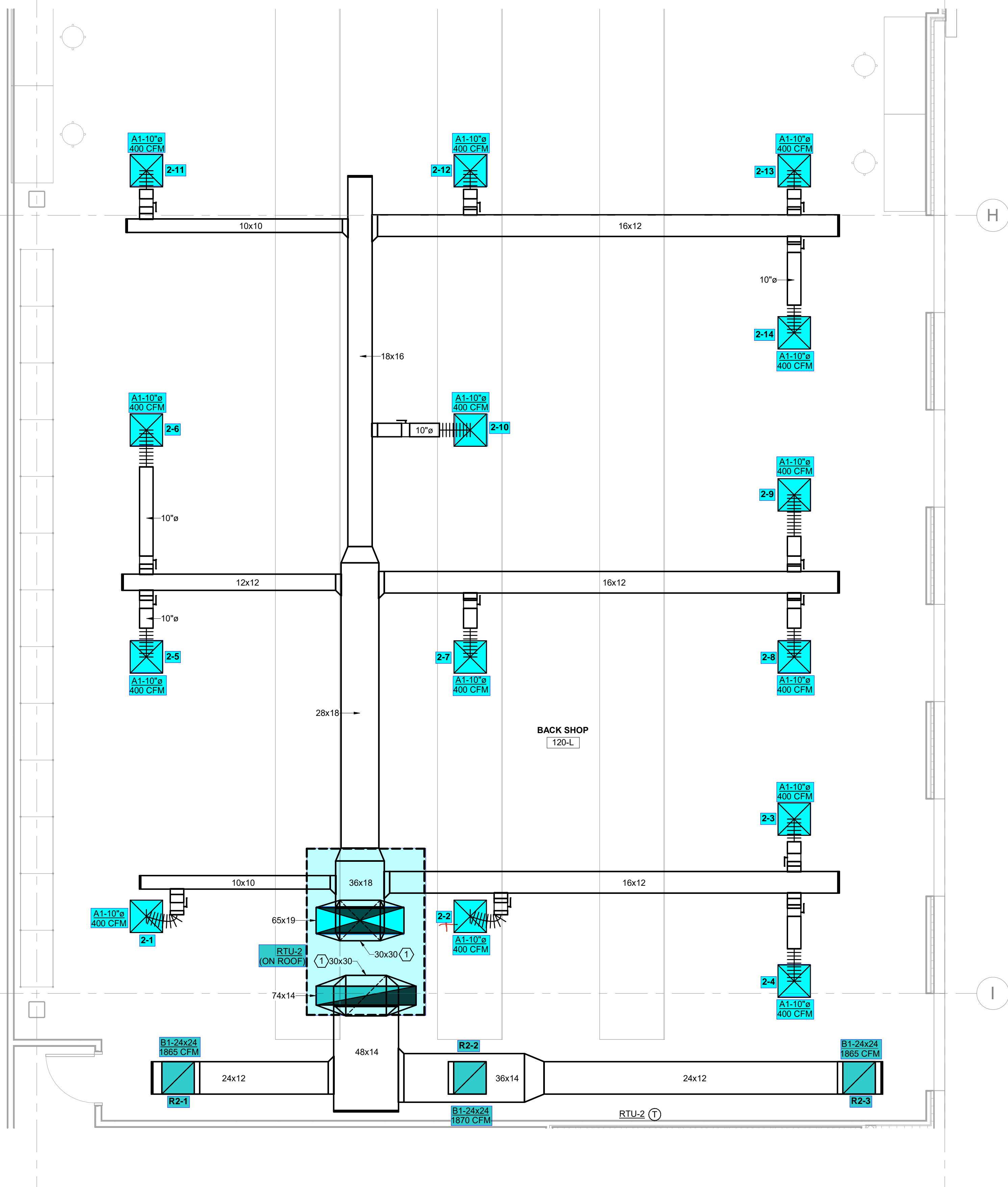
② ENLARGED HVAC PLAN - NEW WORK 1/4" = 1'-0"
