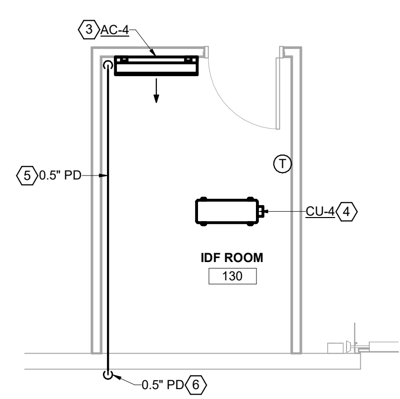
② ENLARGED HVAC PLAN - NEW WORK 1/4" = 1'-0"
